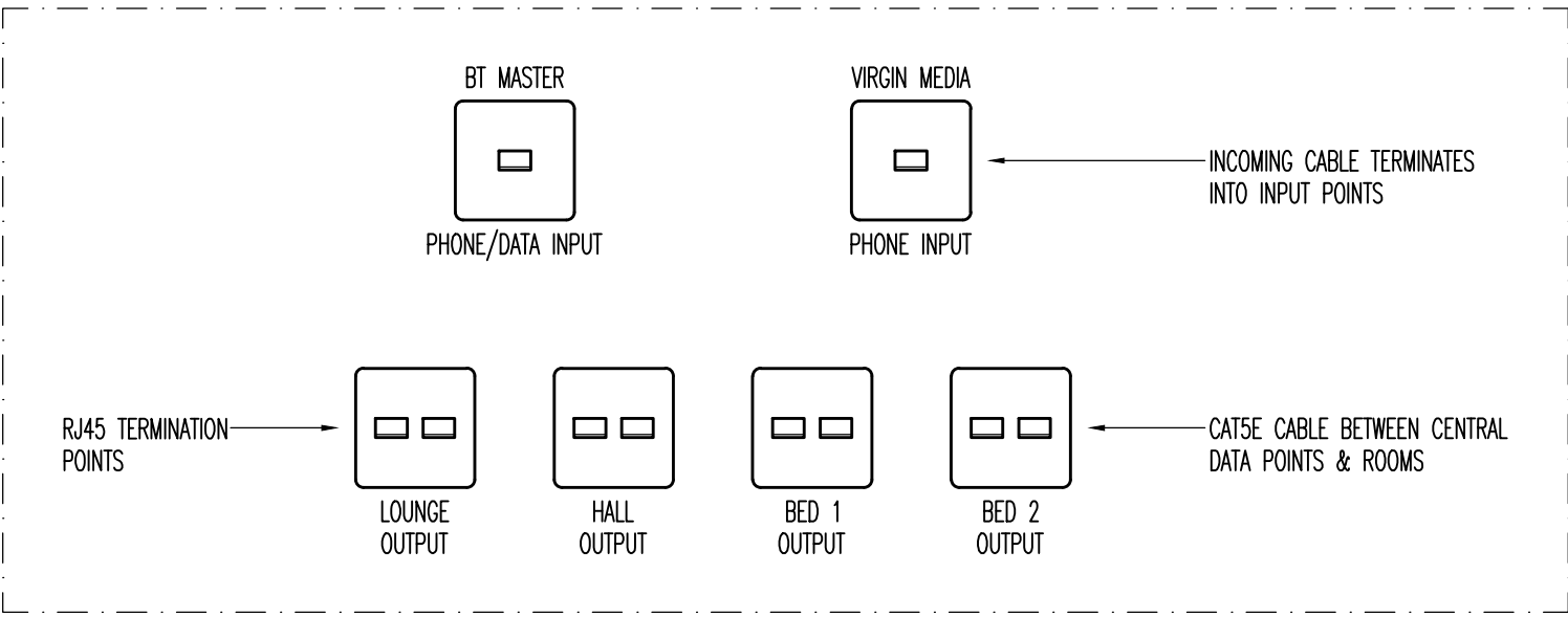
TYPICAL CENTRAL FLAT DATA POINT N.T.S.
