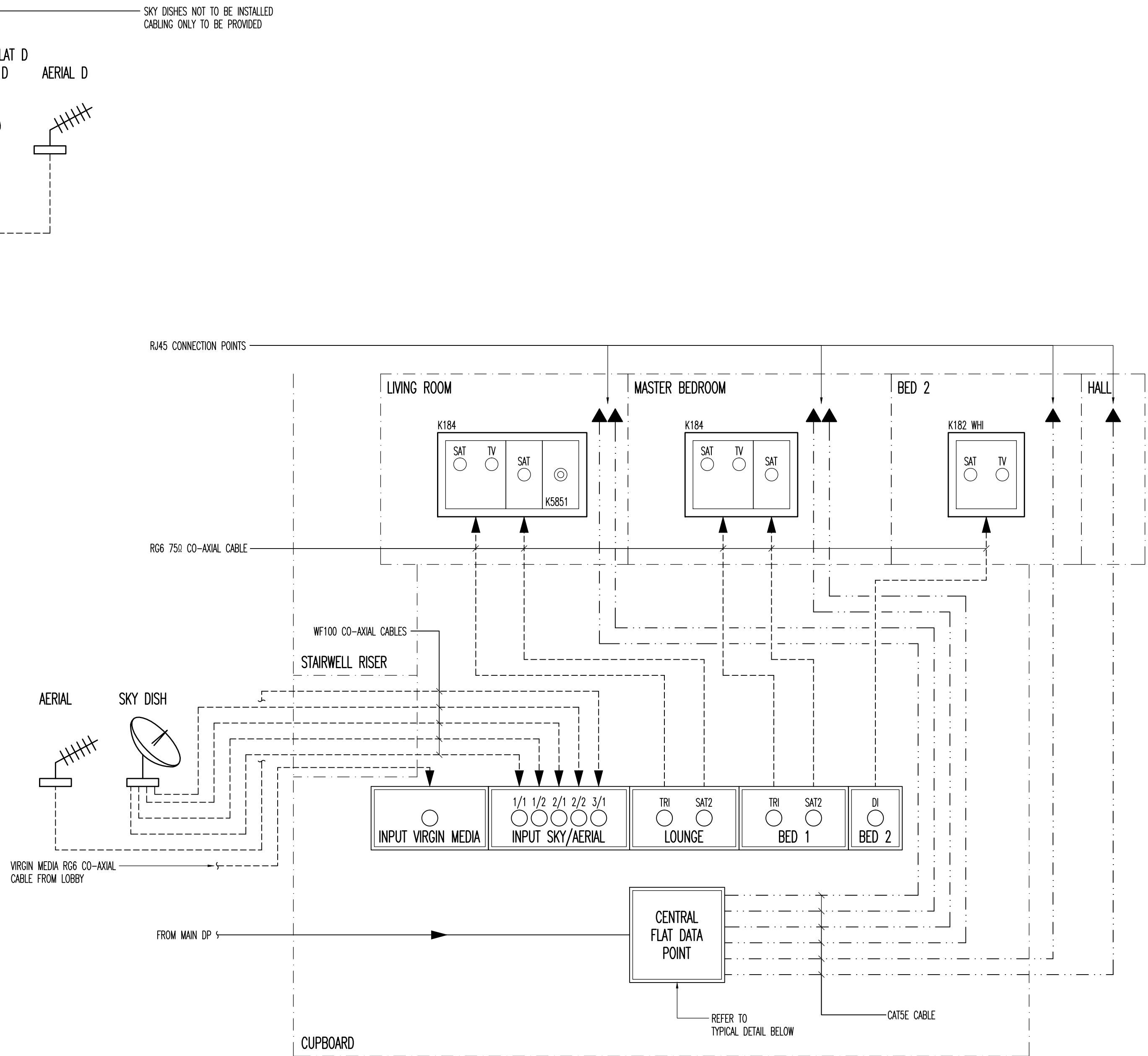
TYPICAL FLAT TV/DATA SCHEMATIC N.T.S.
