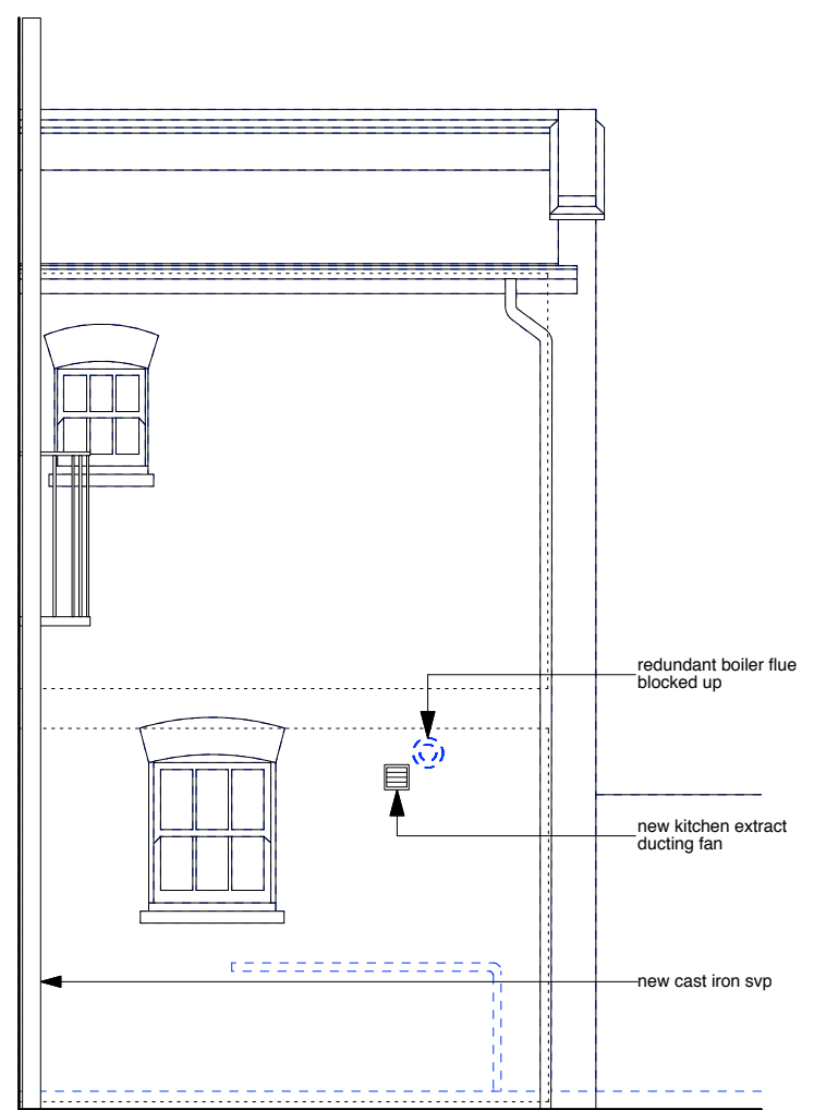
BACK EXTENSION SIDE ELEVATION
