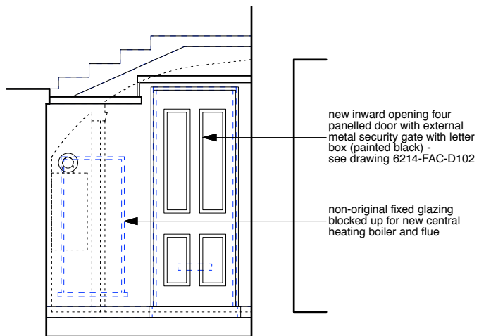
PROPOSED FRONT AREA ARRANGEMENT - SIDE ELEVATION (RAILINGS/BALUSTRADING OMITTED FOR CLARITY)
