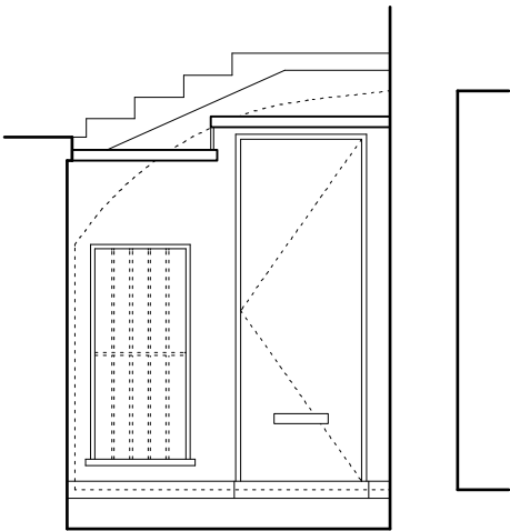
EXISTING FRONT AREA ARRANGEMENT - SIDE ELEVATION (RAILINGS/BALUSTRADING OMITTED FOR CLARITY)
