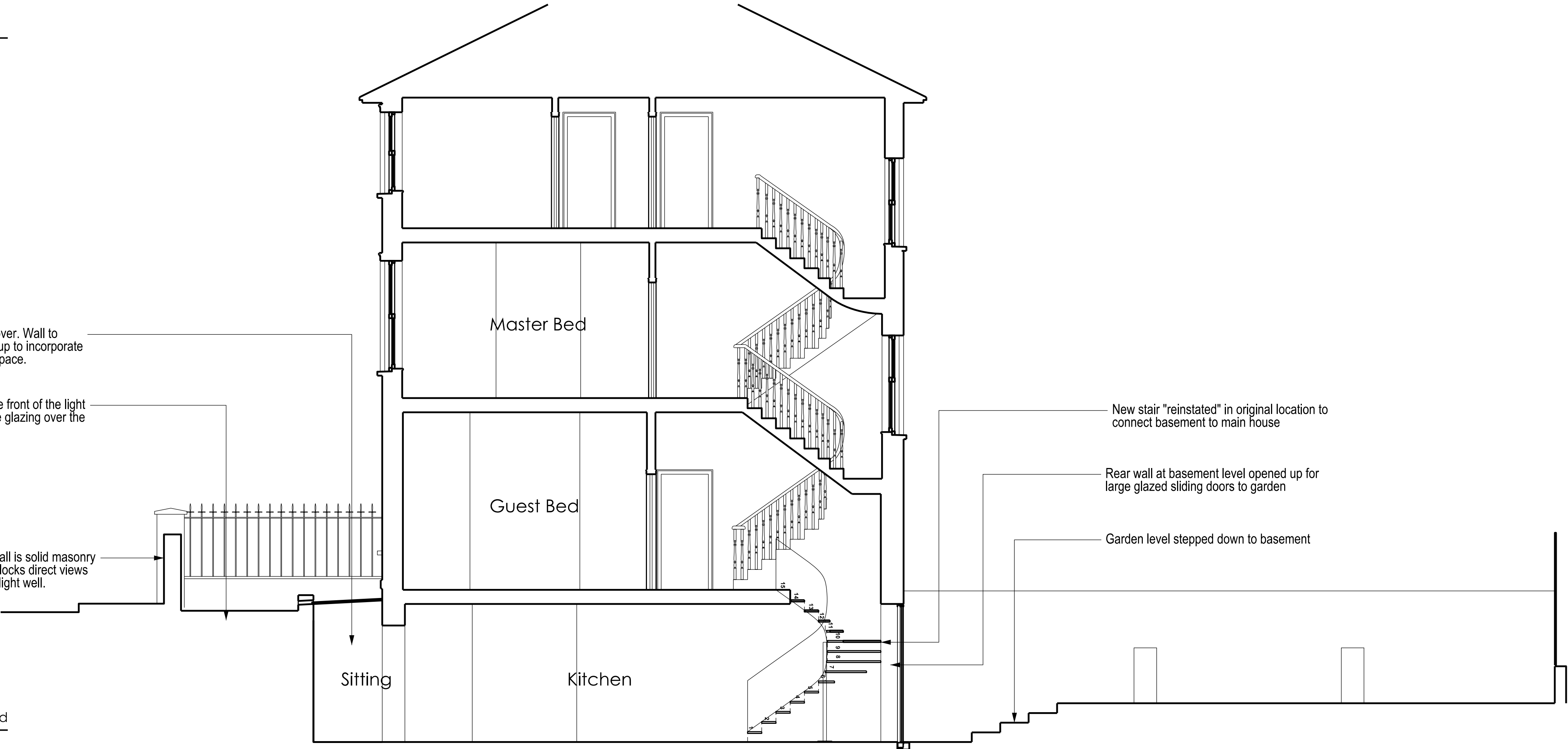
A L04 Section AA - Existing
