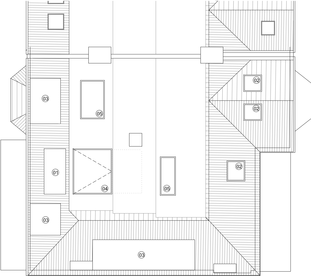
Roof plan
