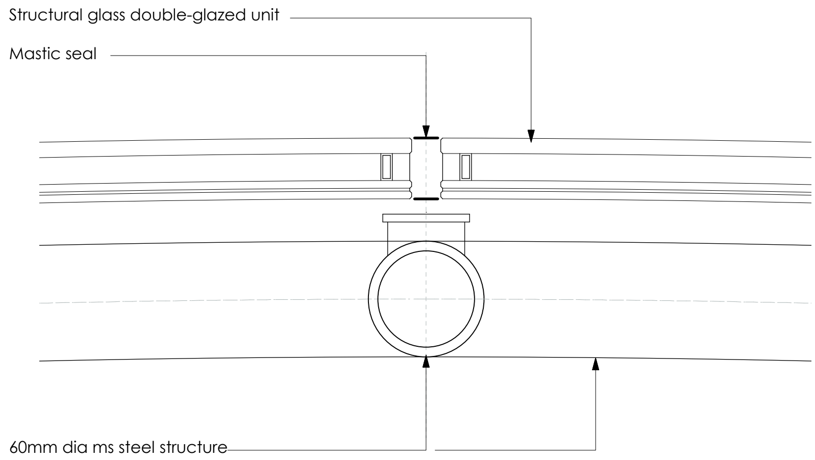
SECTION C-C Scale 1:2
