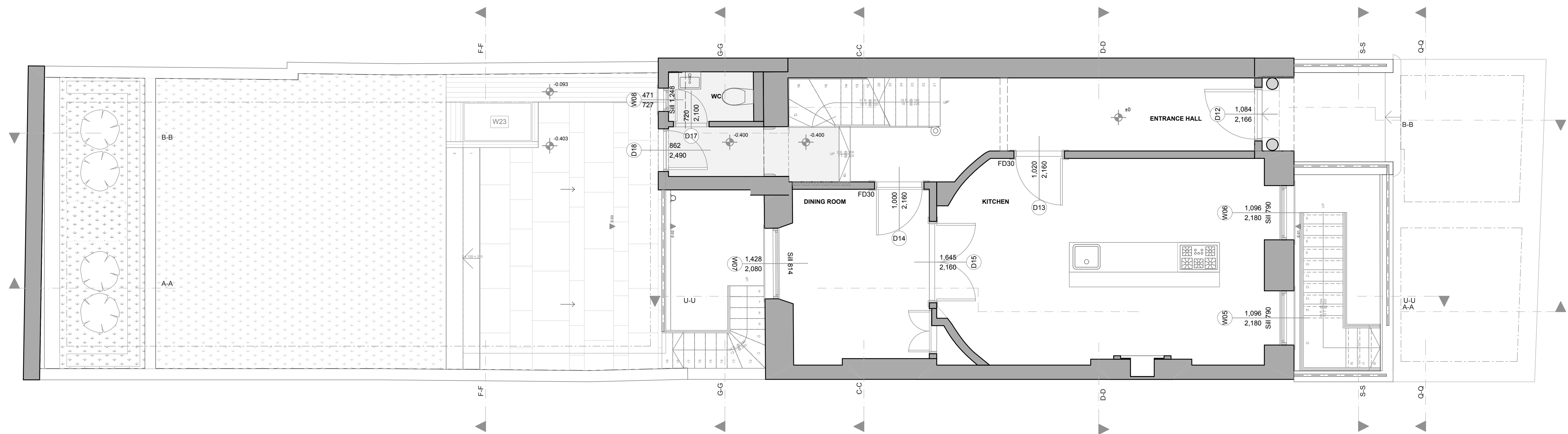
Ground Floor Layout
