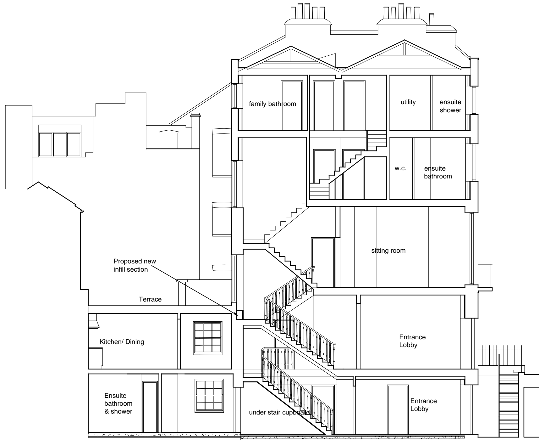
Section C-C
