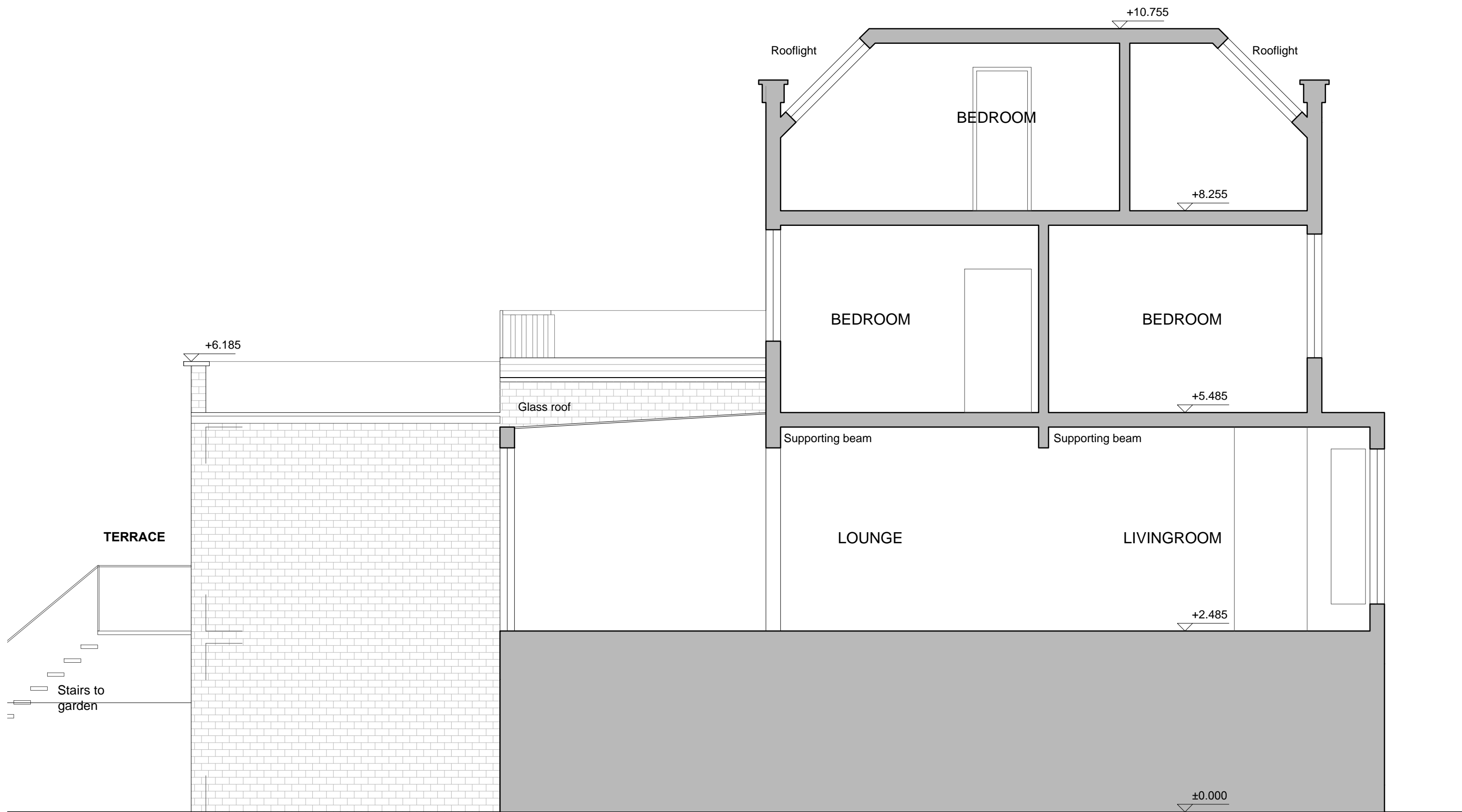
01 EXISTING EAST ELEVATION 1:50
