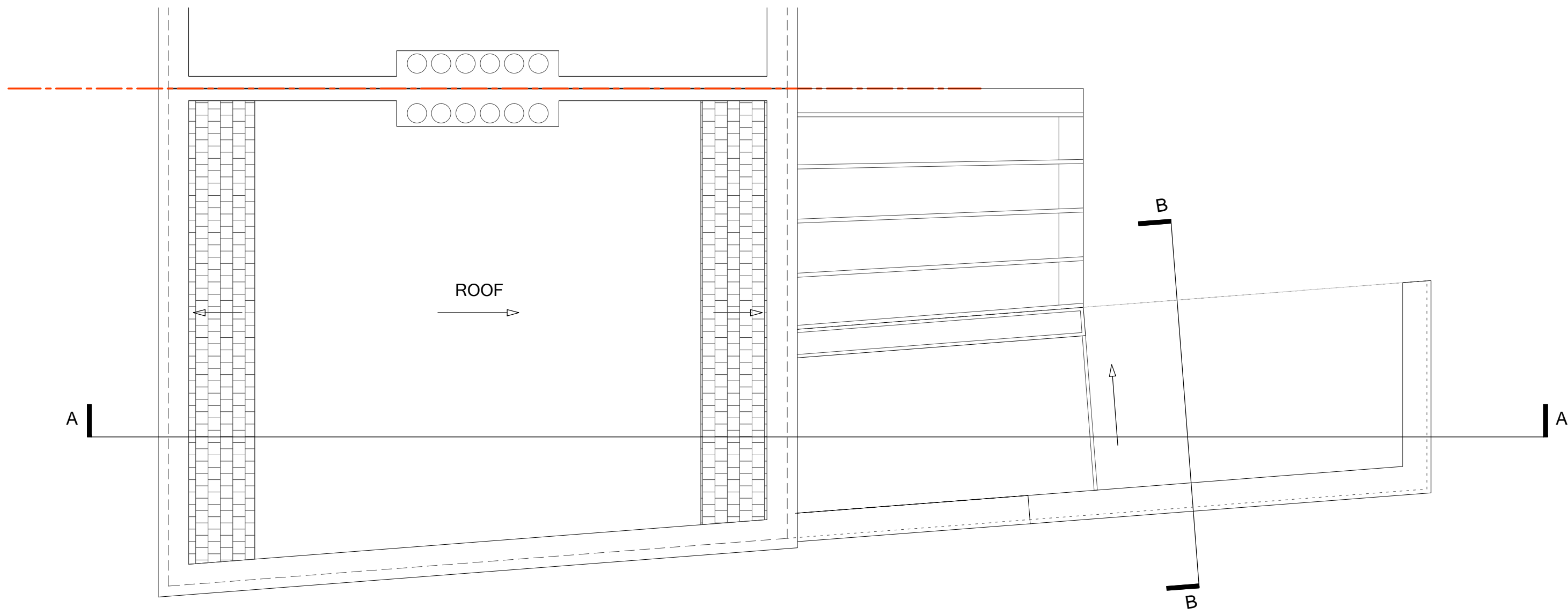
01 EXISTING ROOF PLAN 1:50
