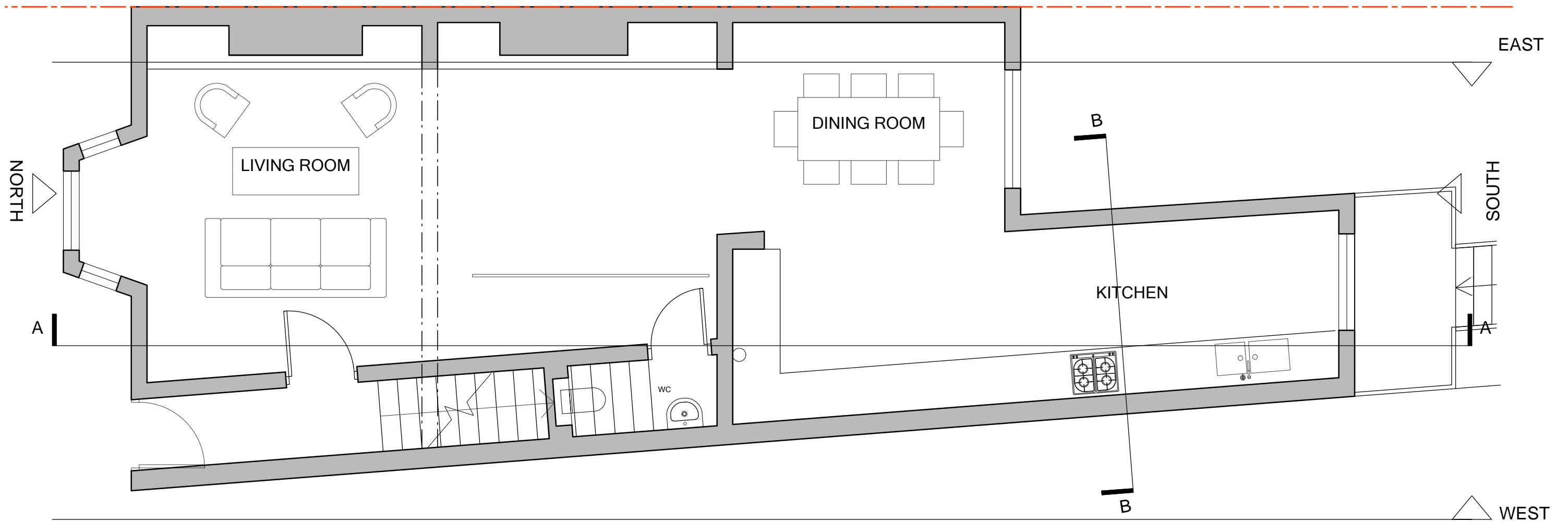
01 EXISTING GROUND FLOOR PLAN 1:50
