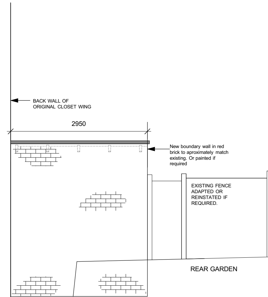
ELEVATION FACING GARDEN OF NO. 2
