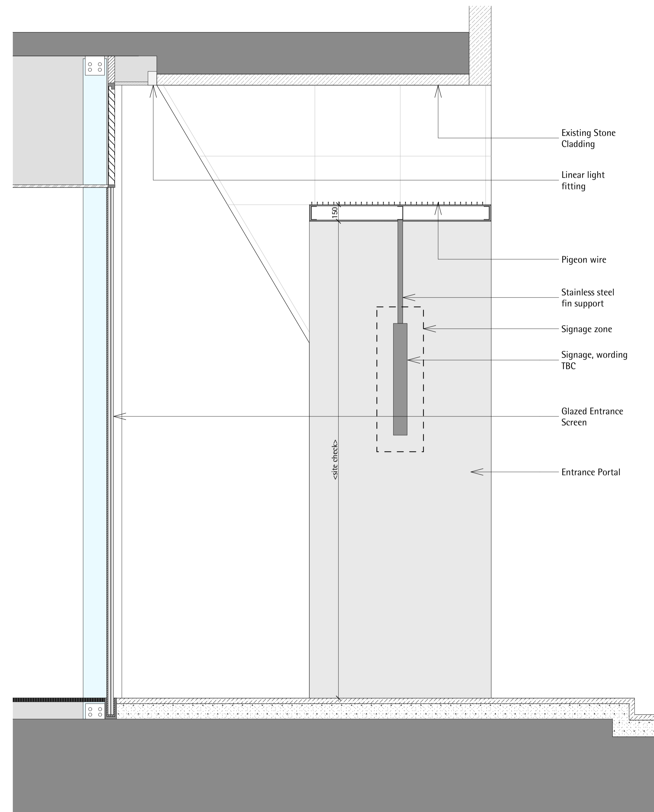
2 Proposed Entrance Signage Section SCALE 1:40
