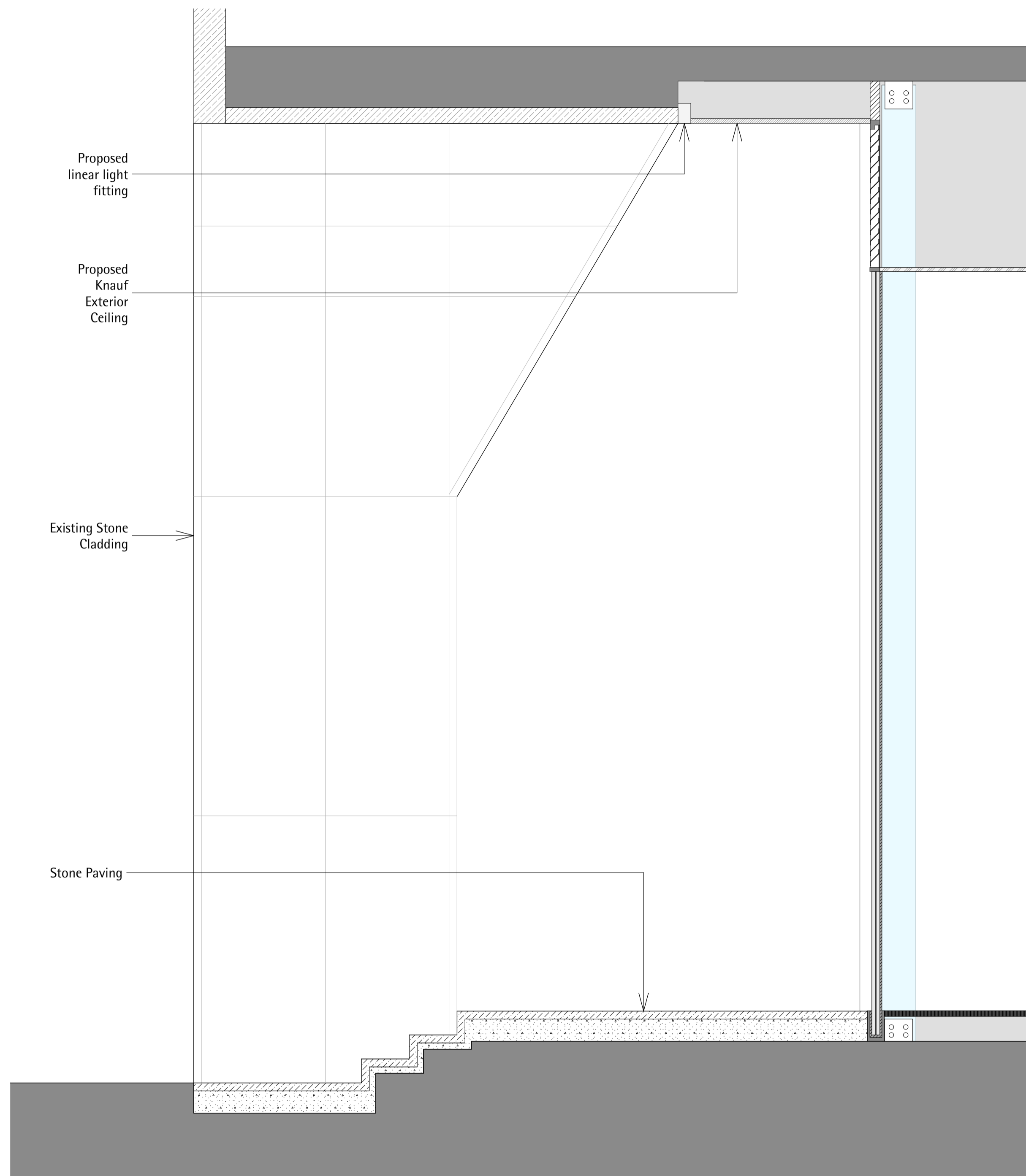
1 Proposed Arcade Soffit Improvements SCALE 1:40
