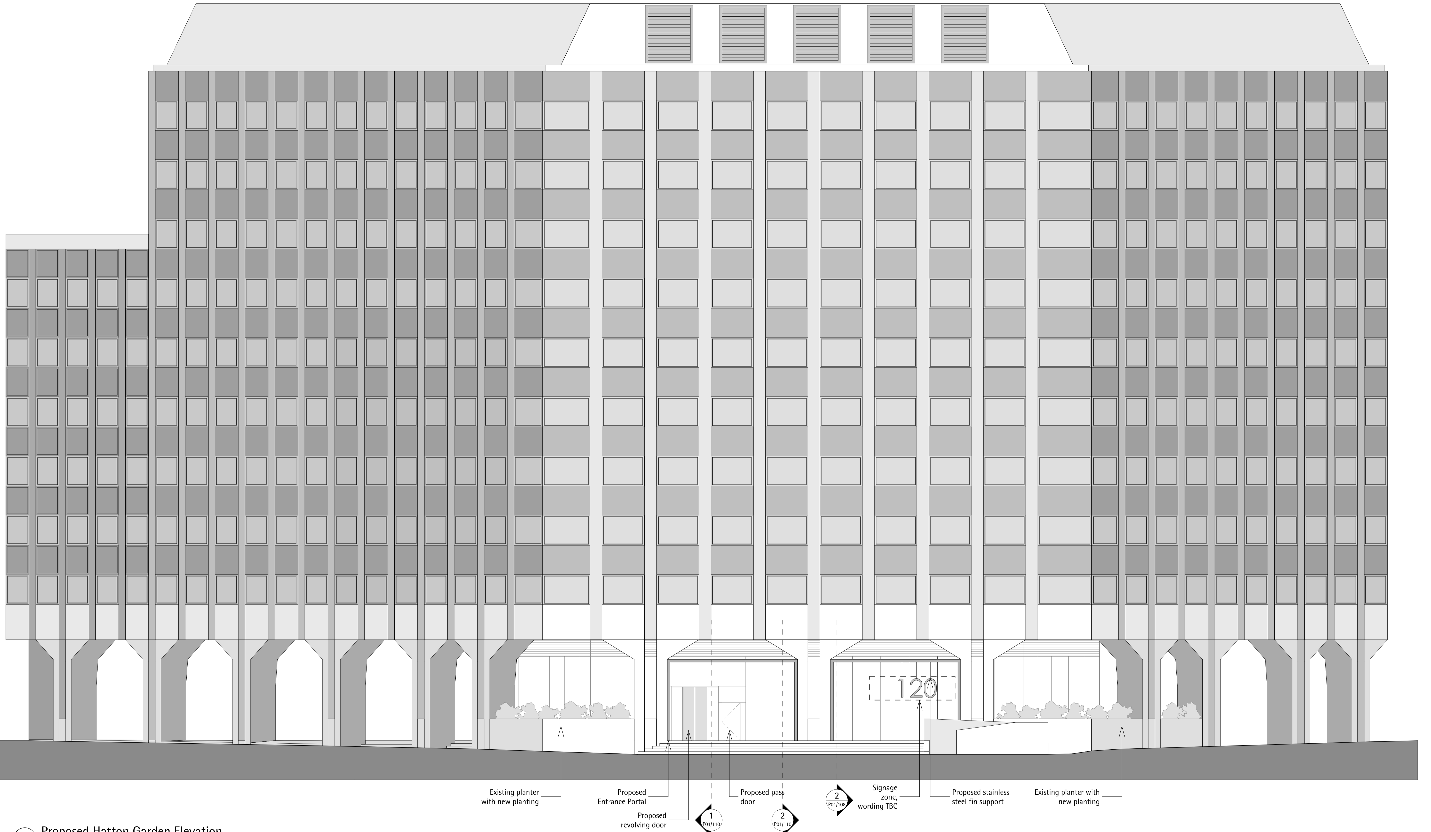
1 Proposed Hatton Garden Elevation SCALE 1:200
