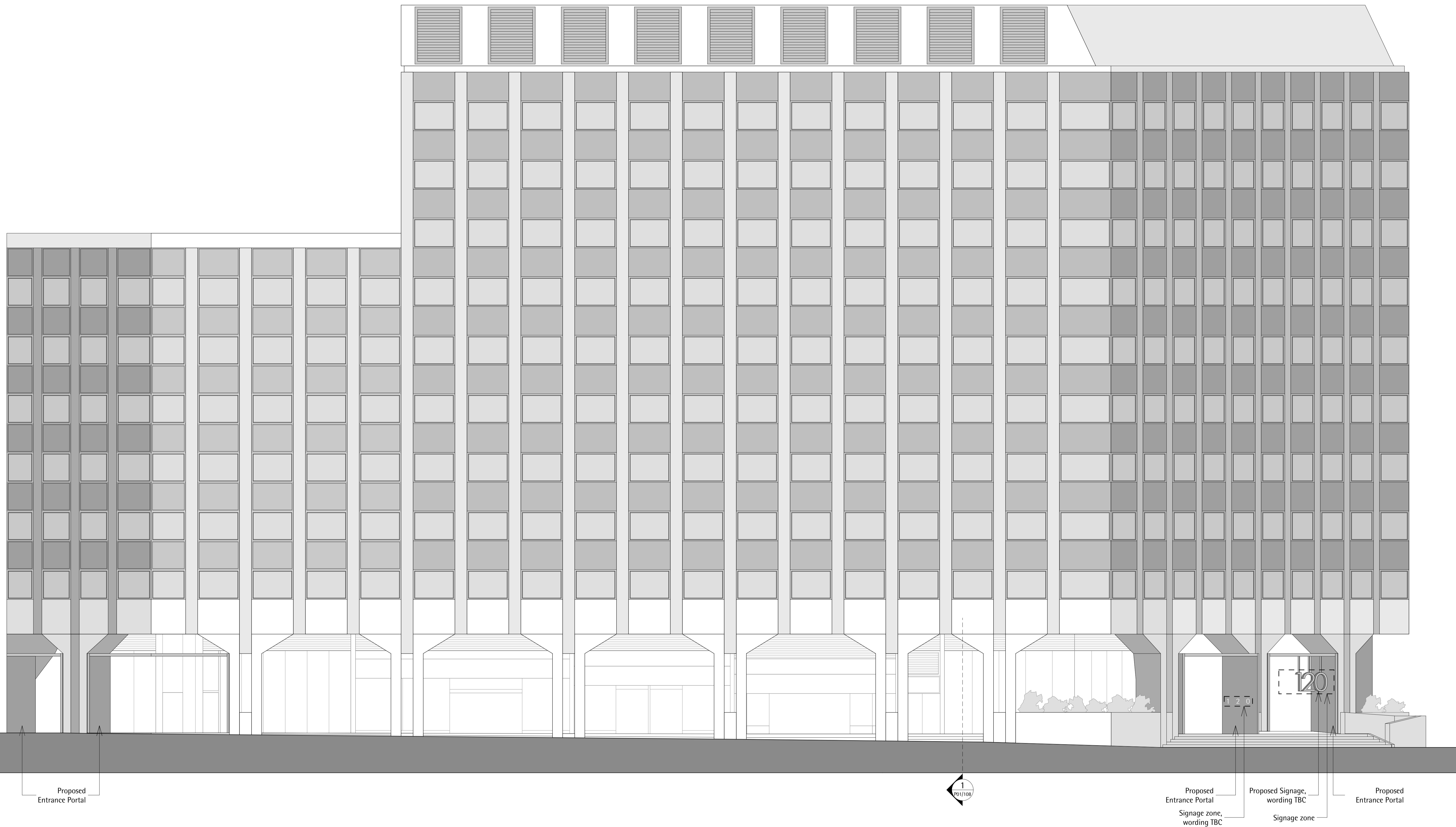
1 Proposed Holborn Elevation SCALE 1:200
