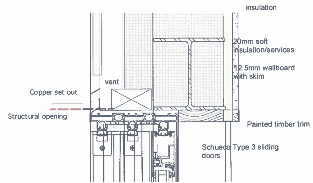
1 Sliding window head Scale: 1:5
