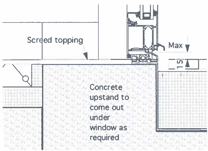
6 Front door threshold Scale: 1:5
