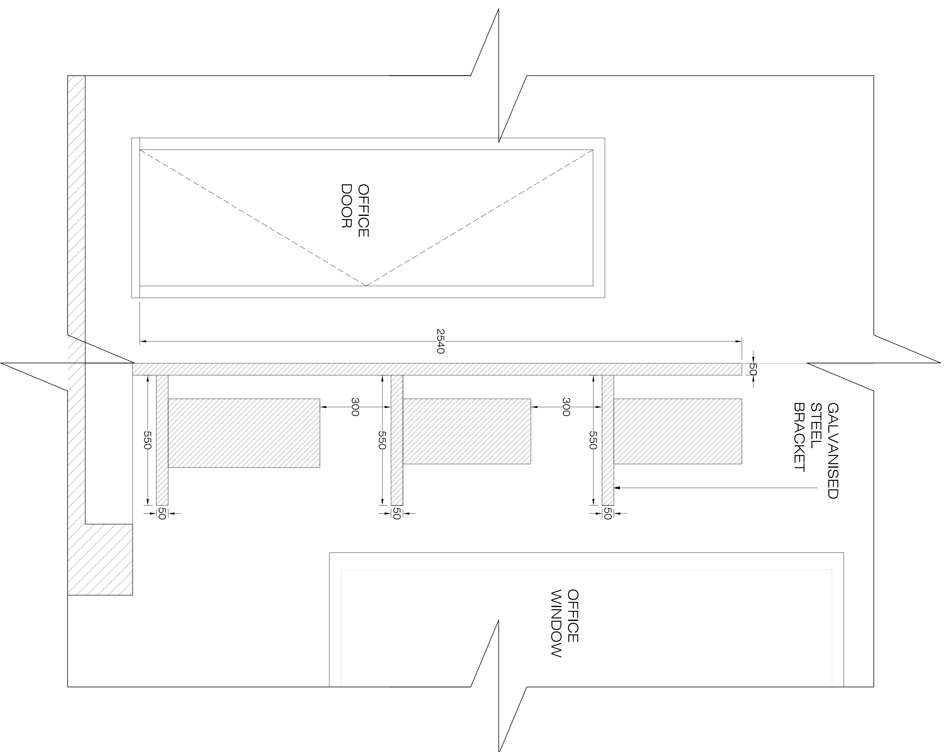
PROPOSED CONDENSER GALVANISED BRACKET DETAIL 02 SCALE 1:20@A3 C-PP-02
