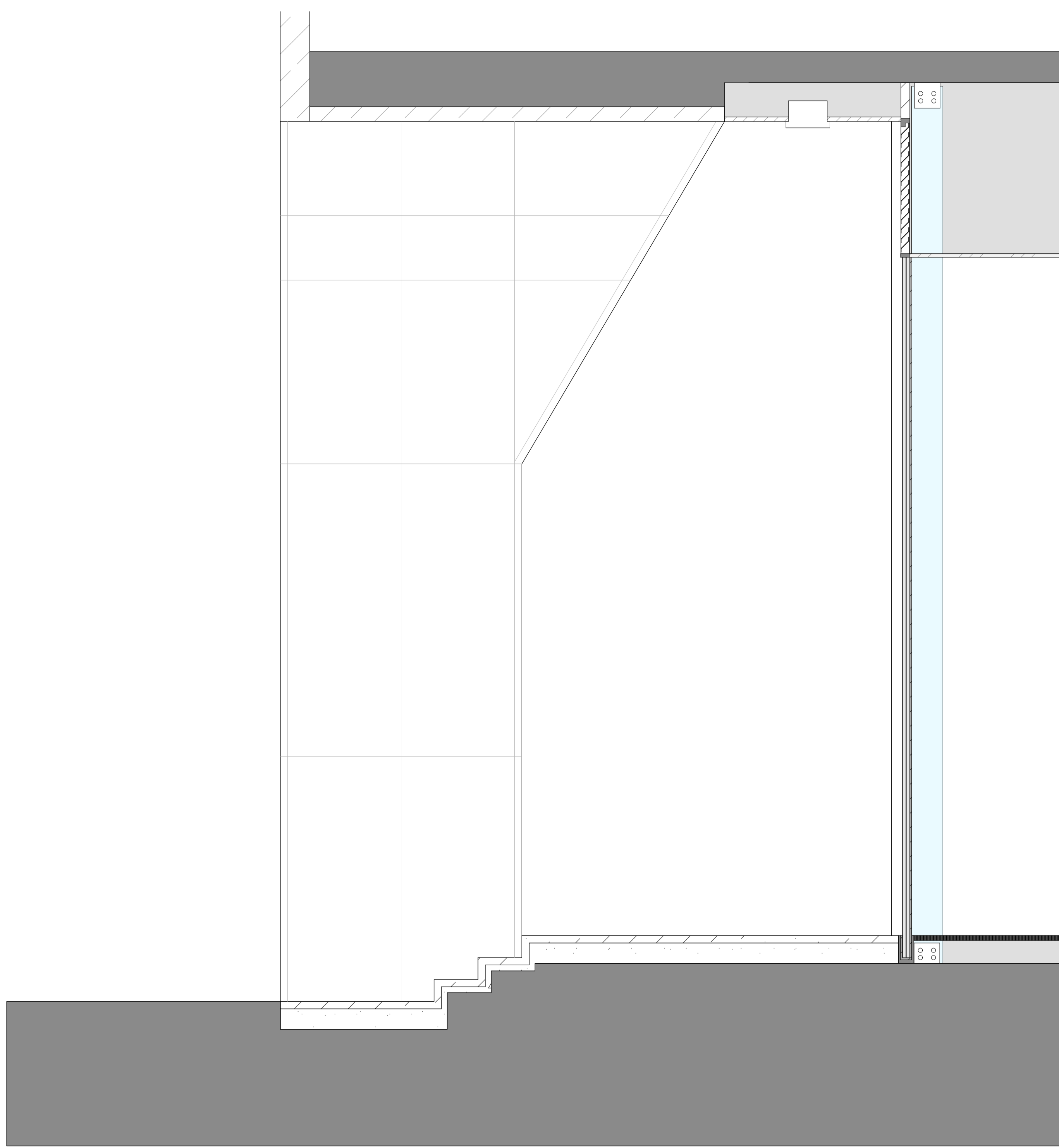
1 Existing Holborn Arcade Section SCALE 1:40
