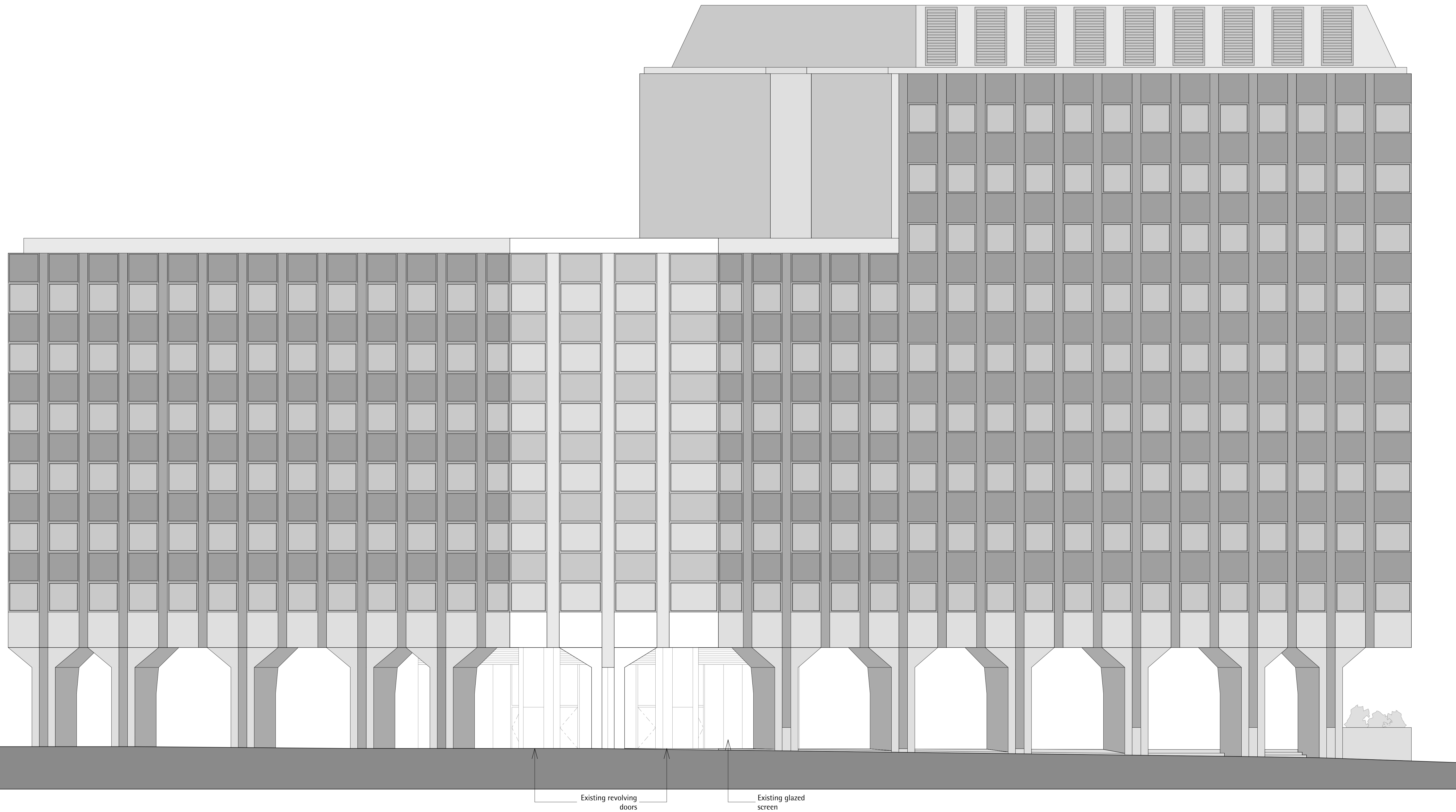
1 Existing Leather Lane Street Elevation SCALE 1:200
