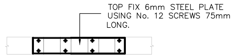
PLAN ON MULTI-NOTCH REPAIR
