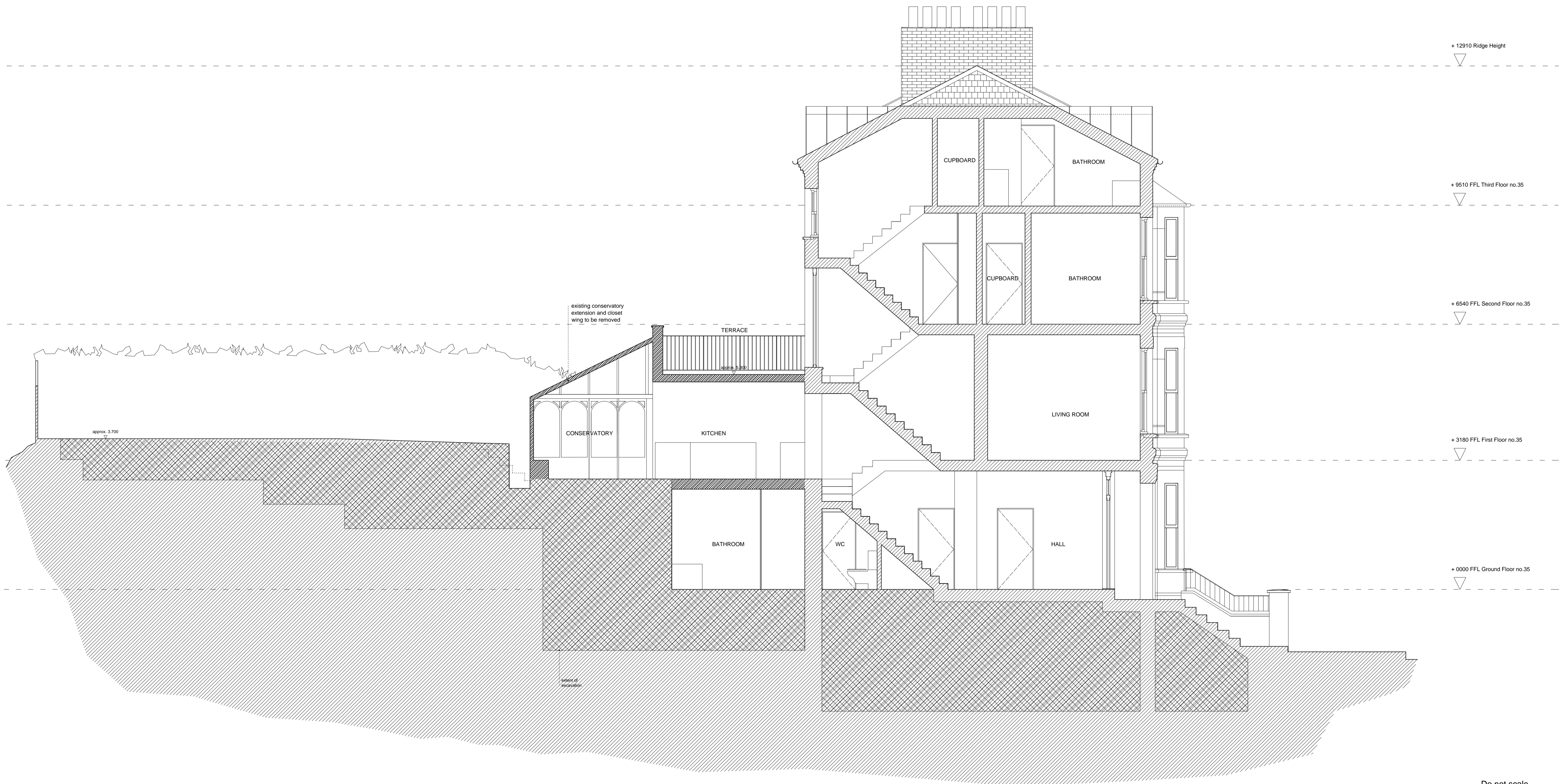
EXISTING SECTION C-C
