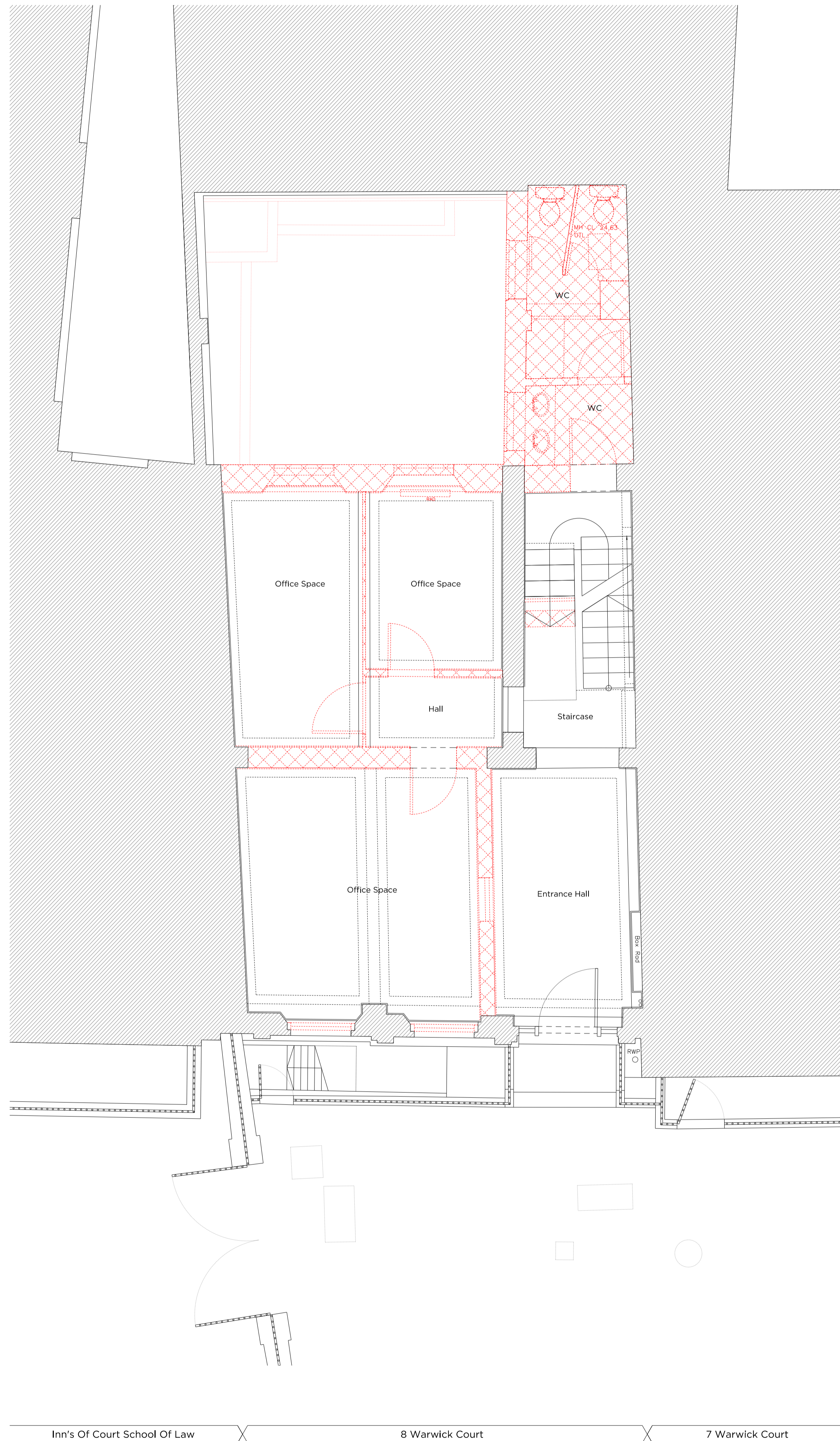
DEMOLITION GROUND FLOOR
