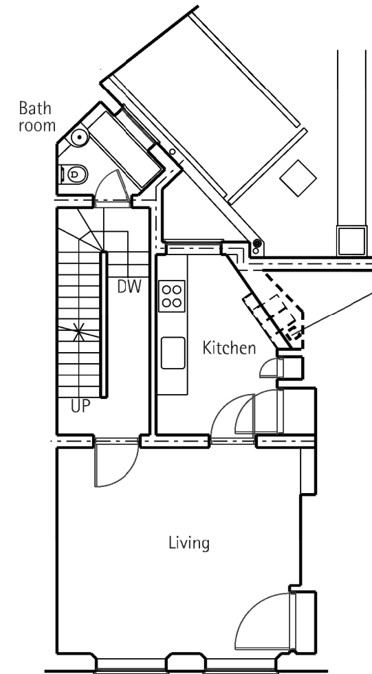
3. Existing first floor plan 1:100 Scale 1:100 @A3
