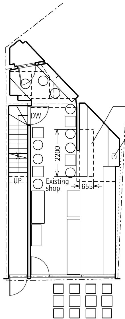
2. Existing ground floor plan 1:100 Scale 1:100 @A3
