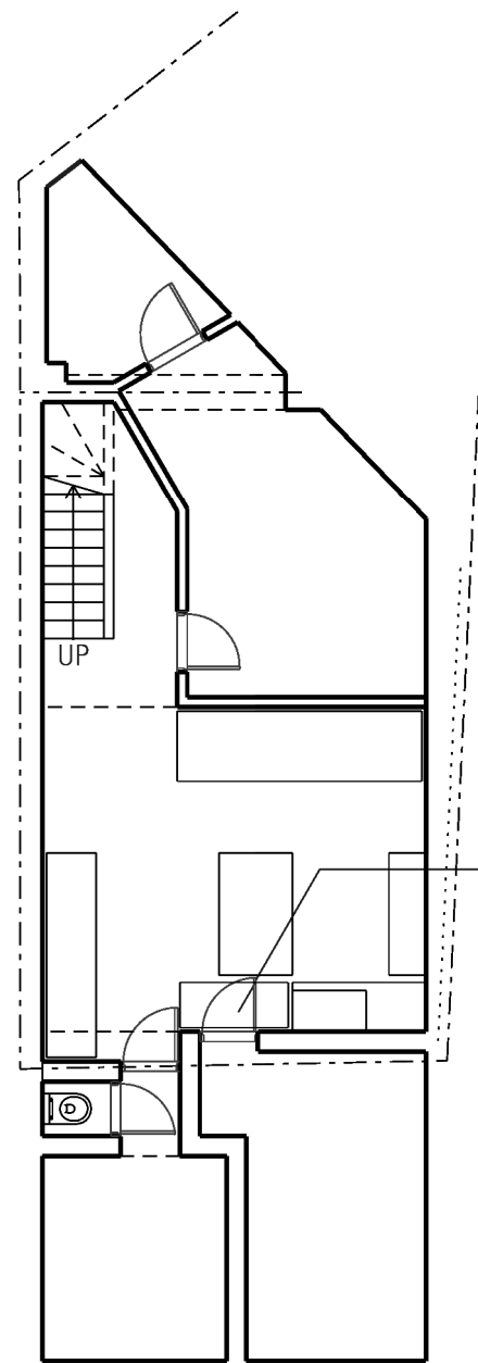
1. Existing basement plan 1:100 Scale 1:100 @A3
