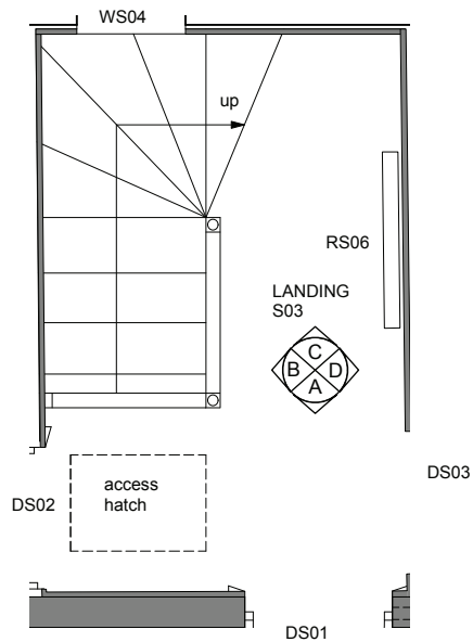
01 Top Floor Plan 1:20@A3
