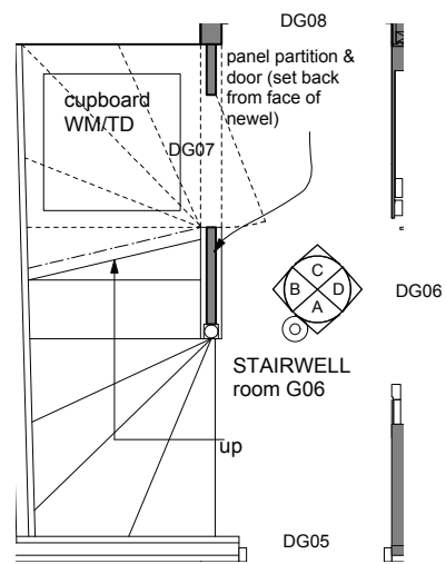
03 Ground Floor Plan 1:20@A3
