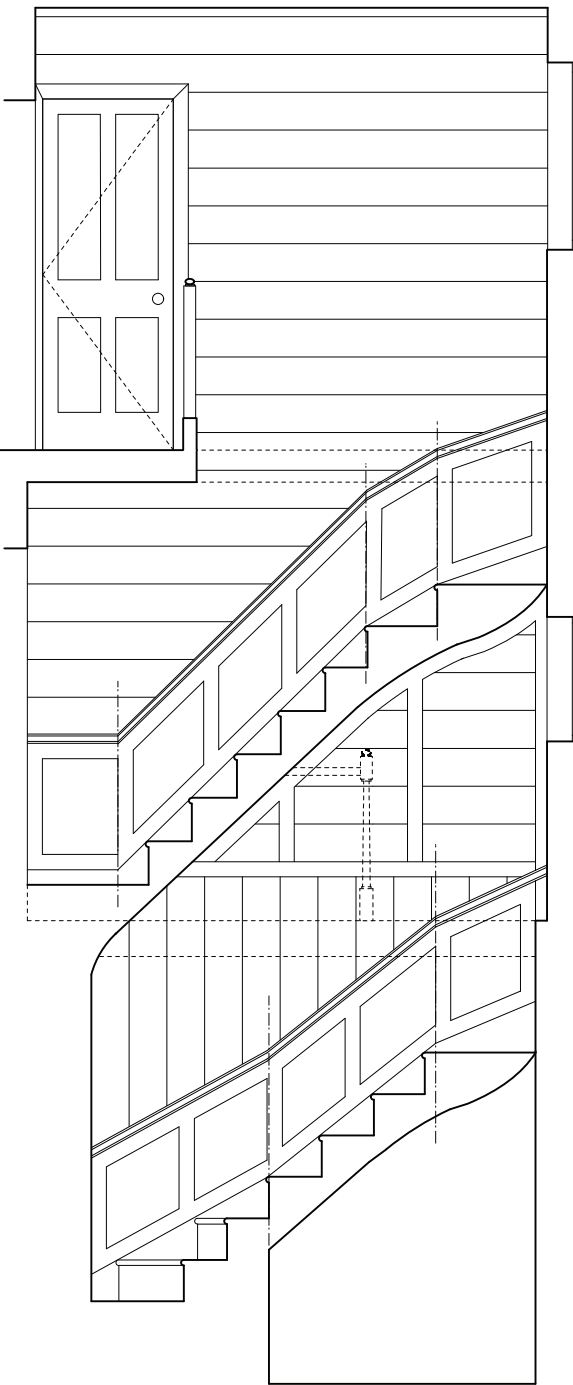
05 Elevation B 1:20@A3
