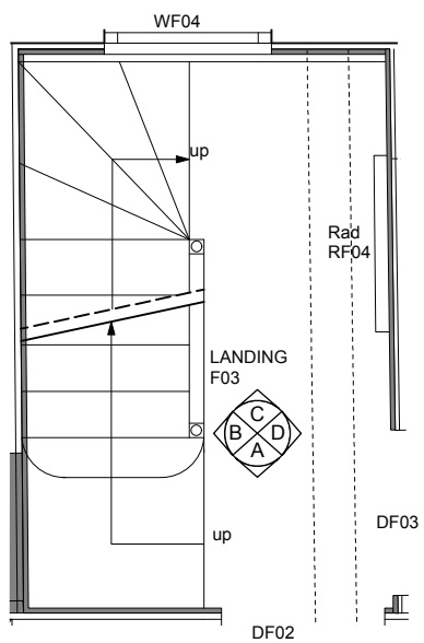
02 First Floor Plan 1:20@A3
