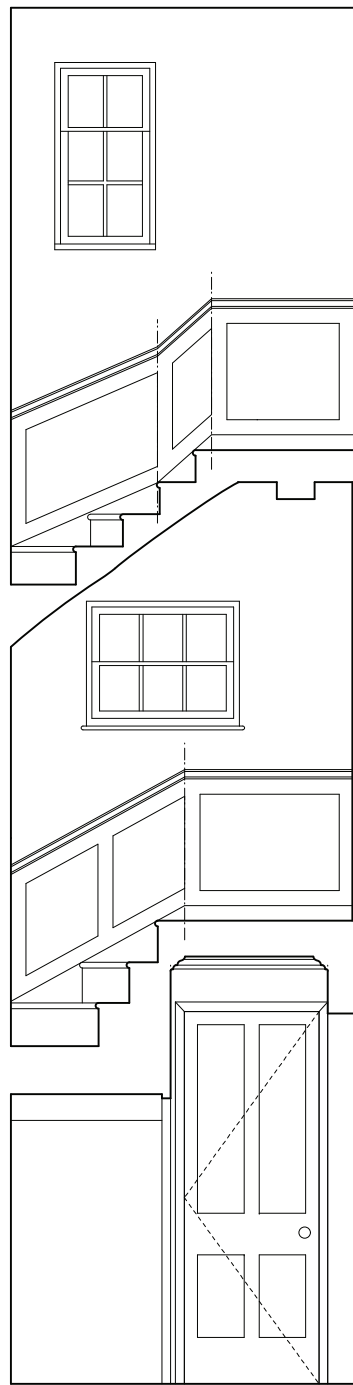
06 Elevation C 1:20@A3
