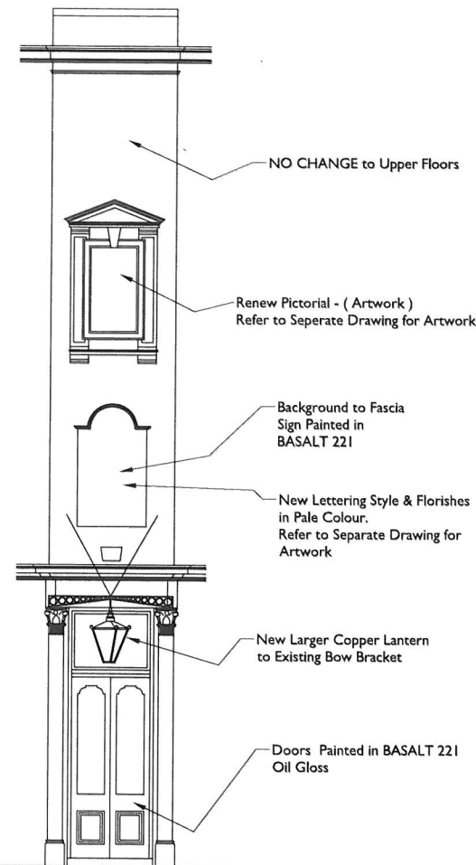
CORNER ELEVATION
