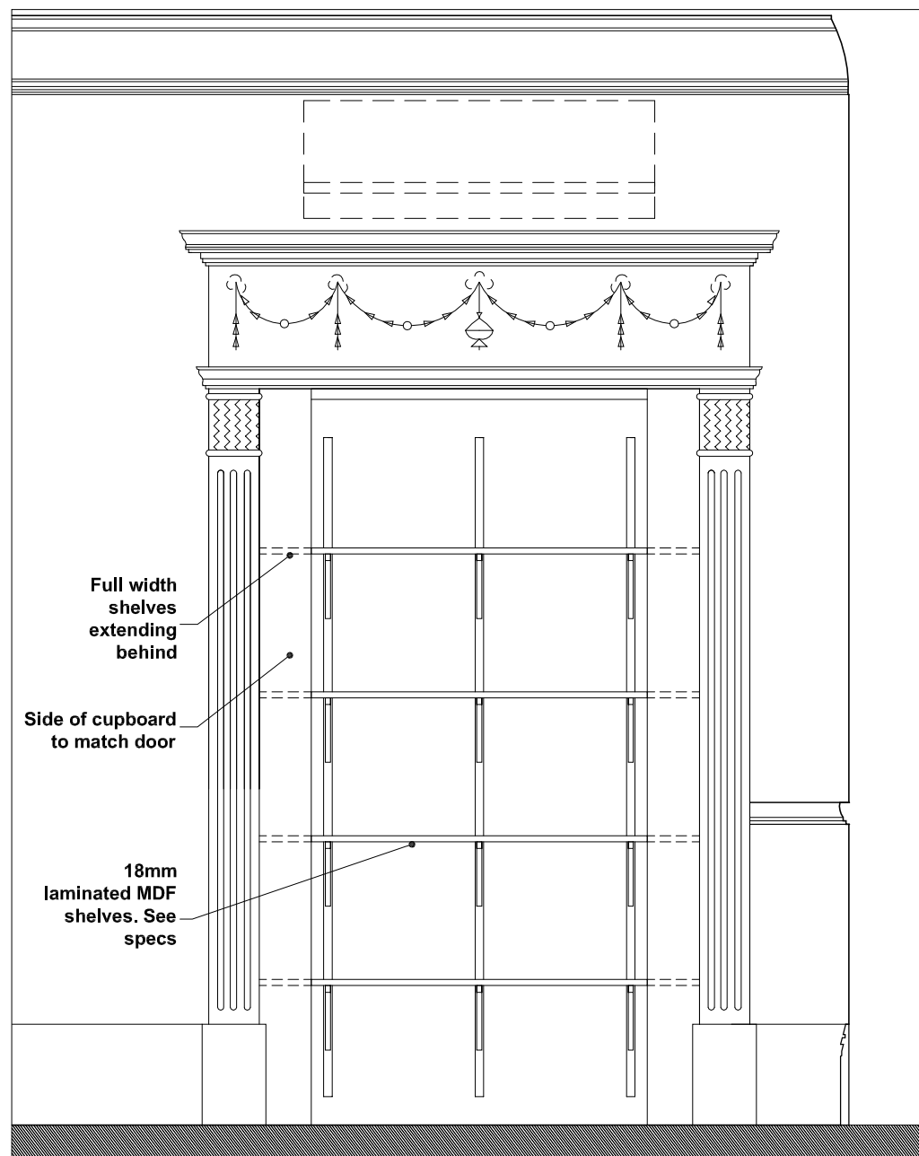
Elevation without doors
