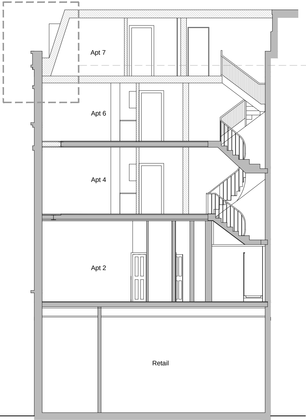
SECTION B-B
