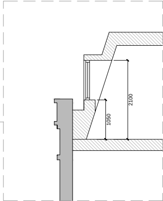
Typical Dormer Arrangement
