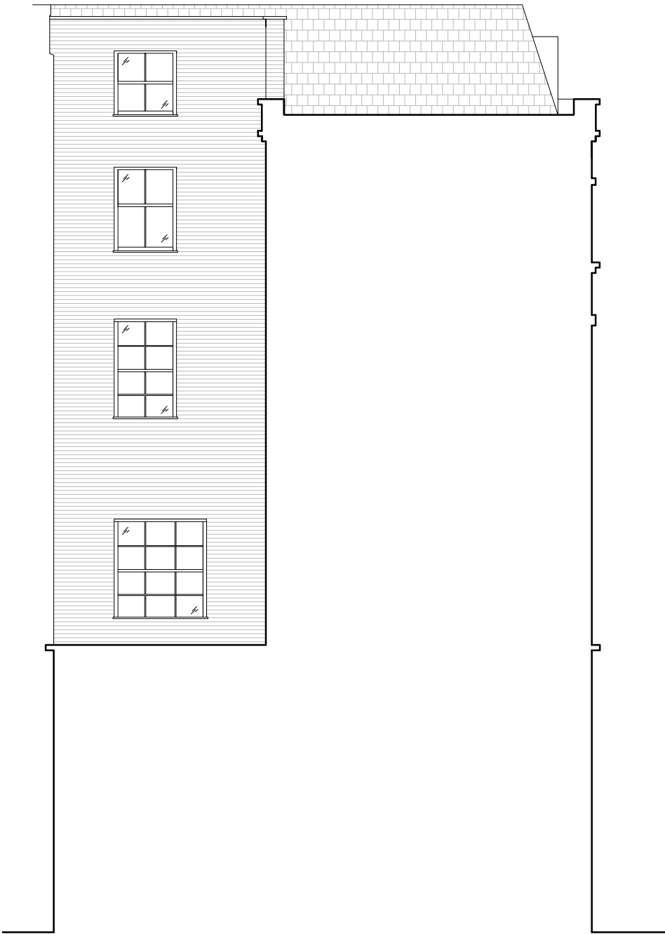
NORTH WEST ELEVATION
