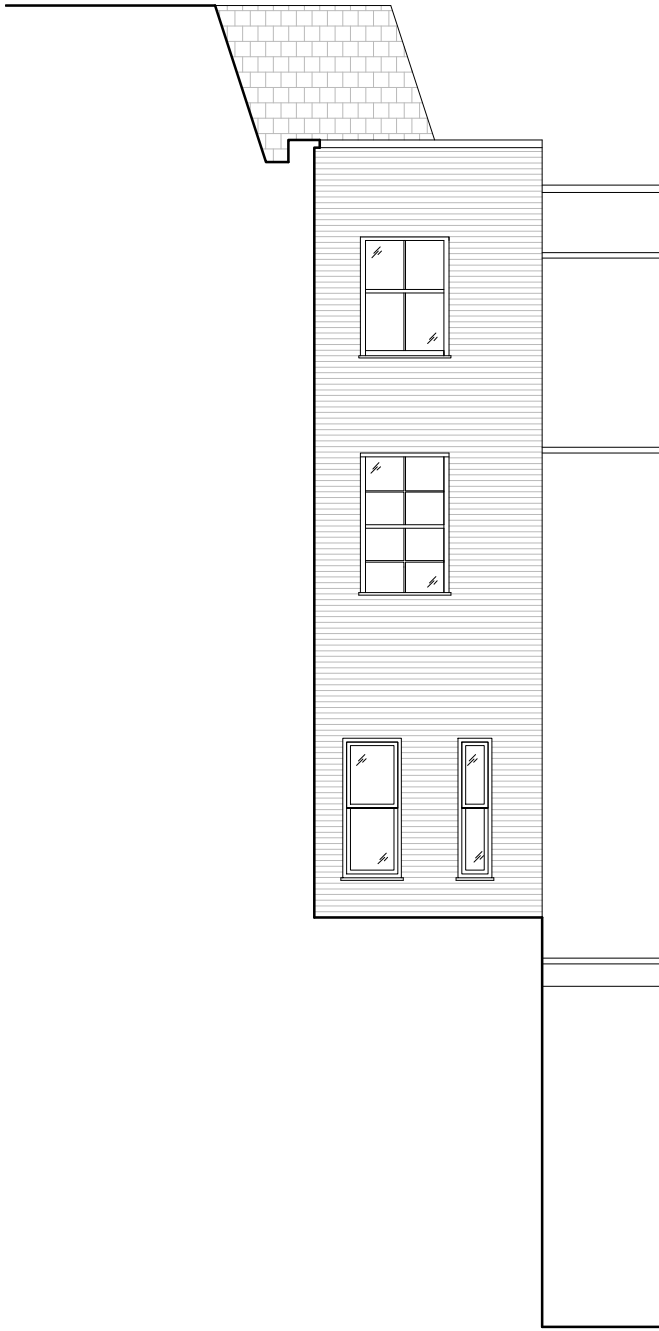
SOUTH WEST REAR ELEVATION
