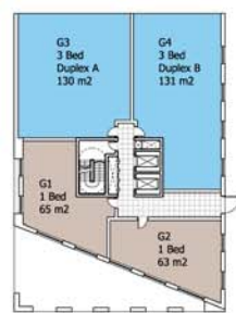
Ground Floor
