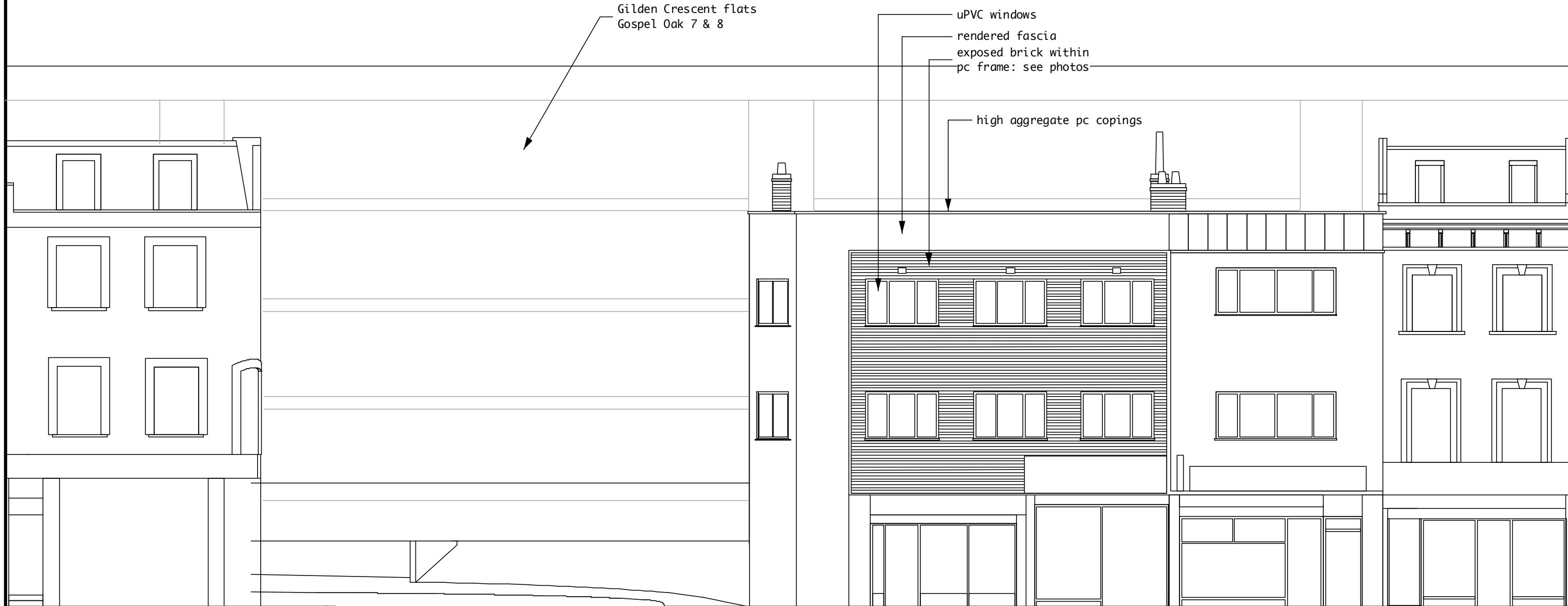
1 existing Queens Crescent elevation Scale: 1:100
