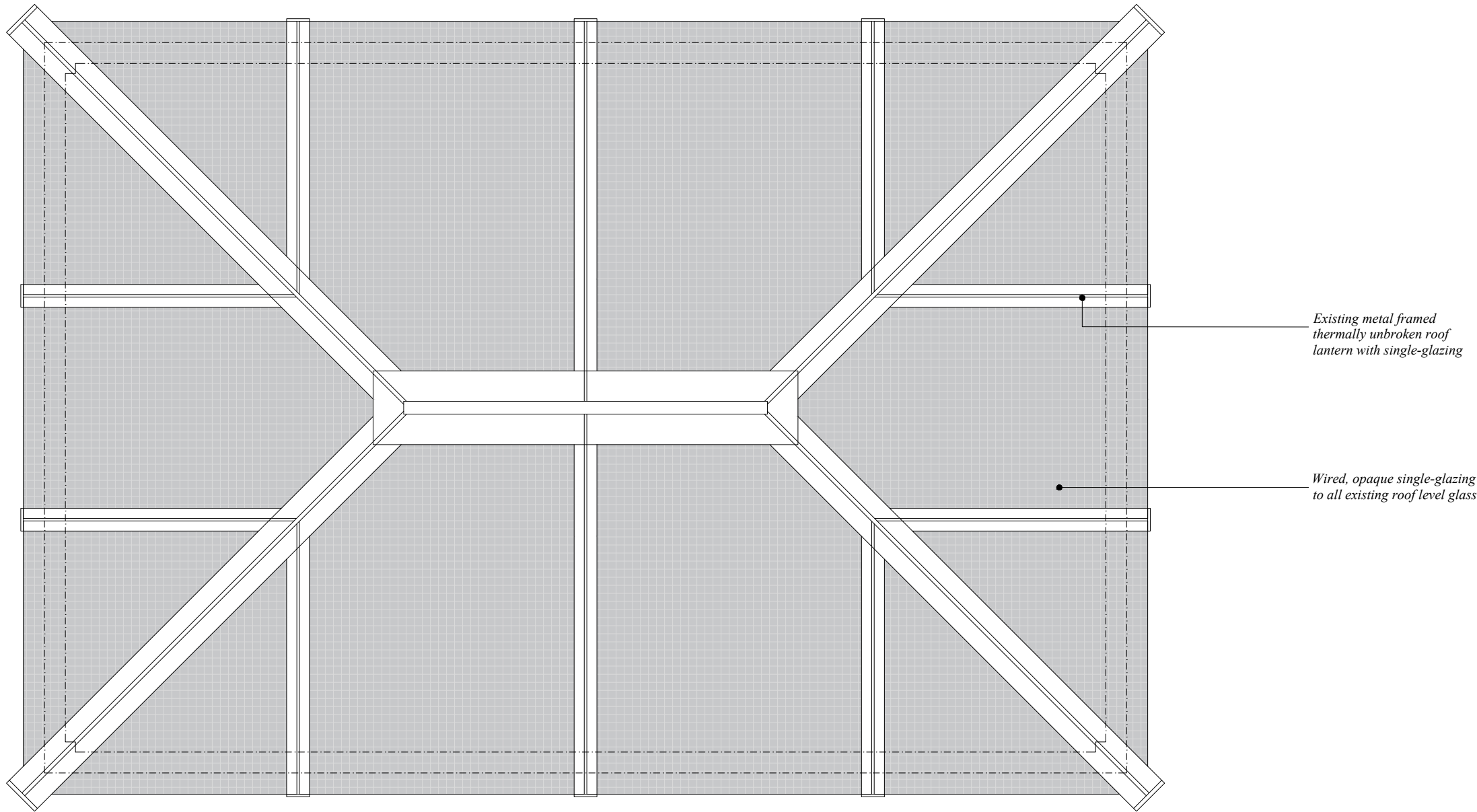
Existing Lantern Roof Plan (Extract)
