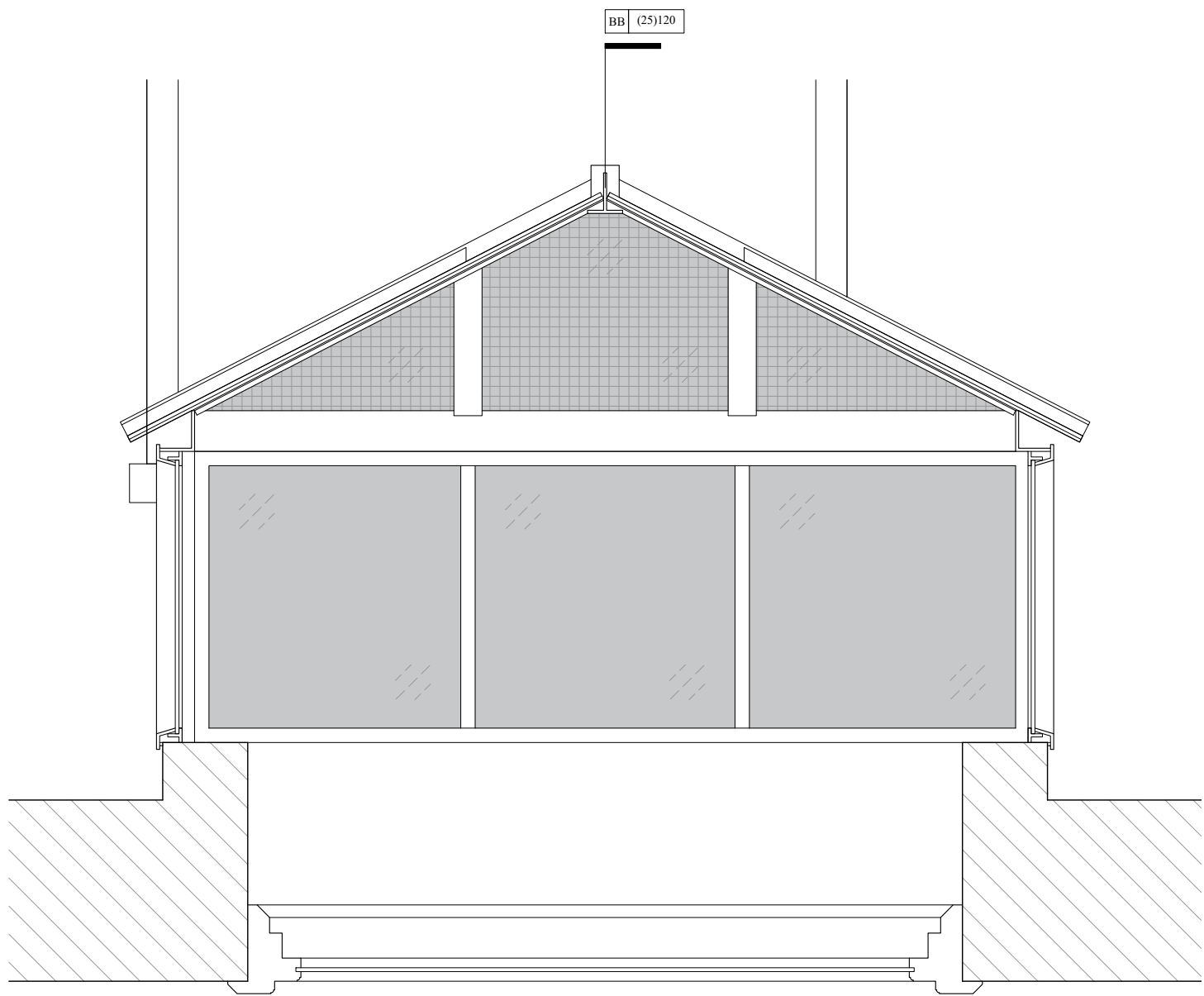
Existing Short Section/ Internal Elevation
