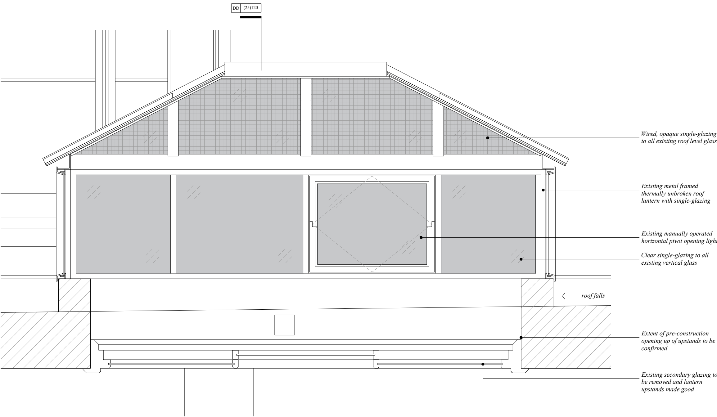
Existing Long Section/ Internal Elevation
