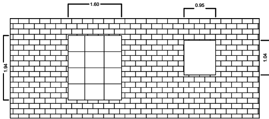
Existing Ground Floor Rear Elevation
