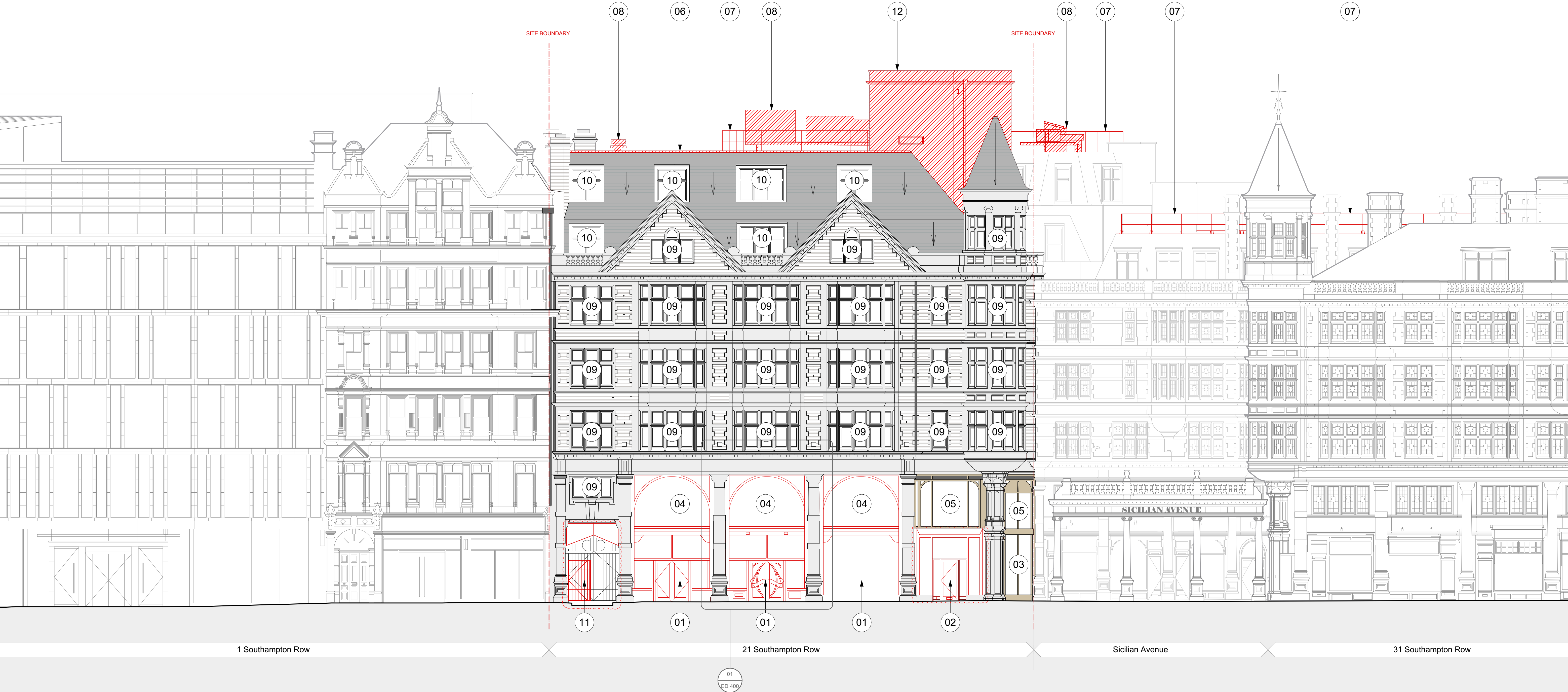
21SR Demolition East Context Elevation Scale: 1:100
