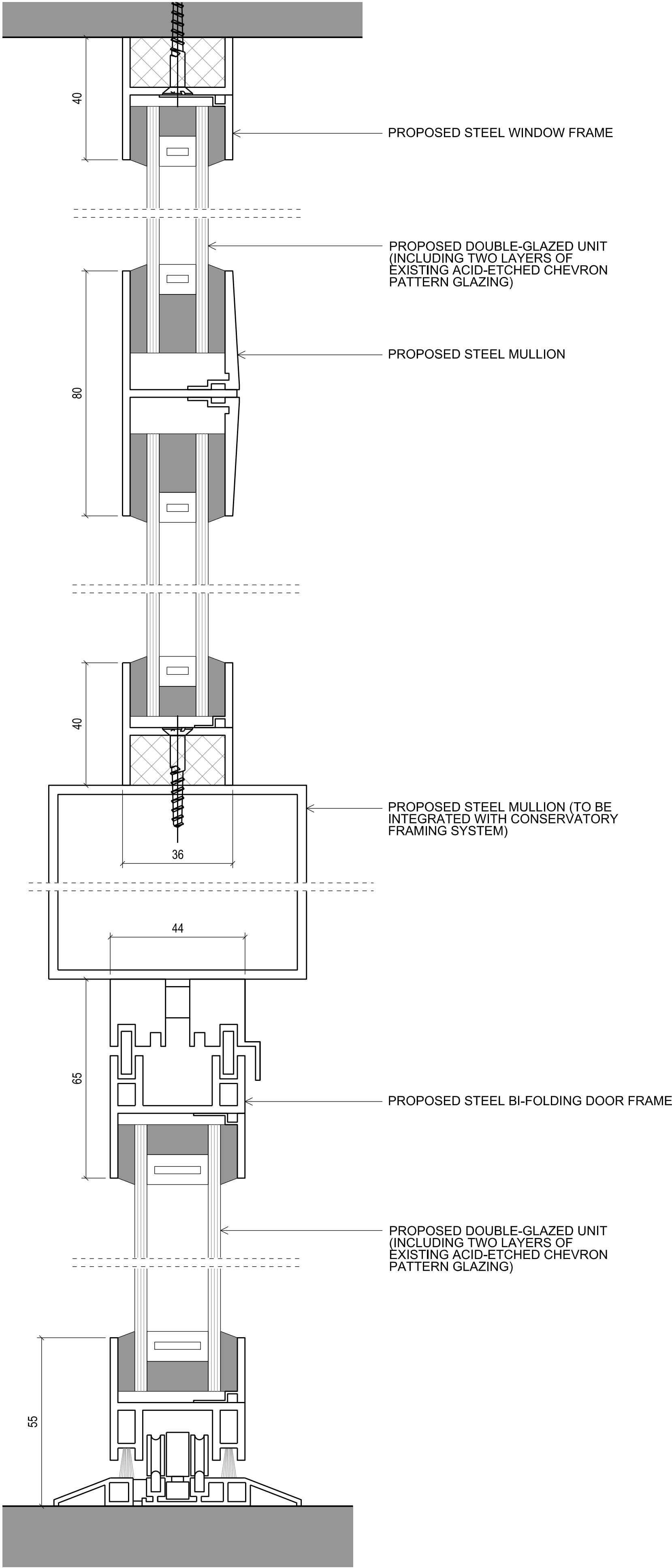
1 PROPOSED WINDOW TYPICAL DETAILS - SECTION A-A Scale 1:2 at A3 / 1:1 at A1
