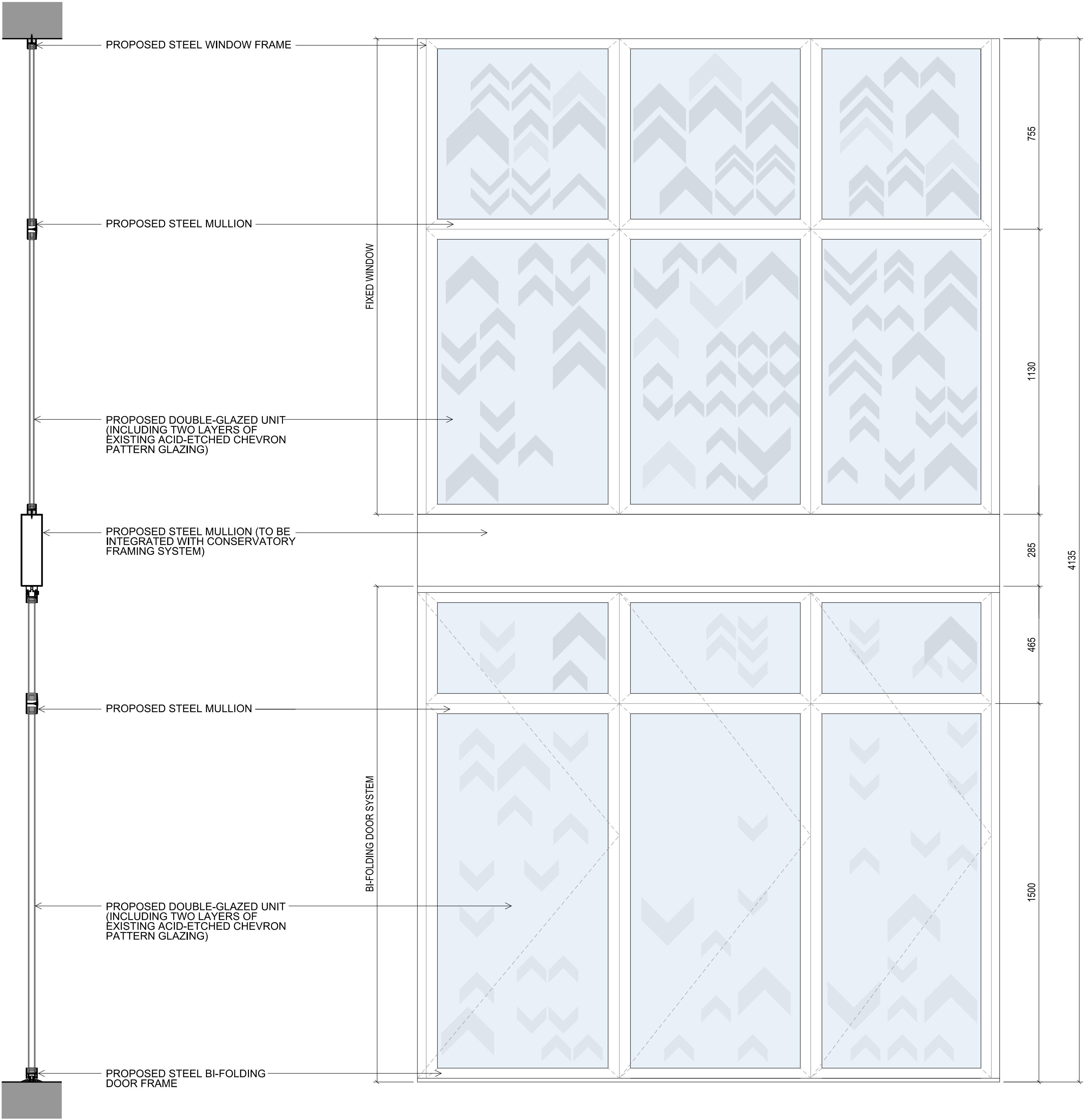
2 PROPOSED WINDOW TYPICAL DETAILS - FULL SECTION Scale 1:20 at A3 / 1:10 at A1
