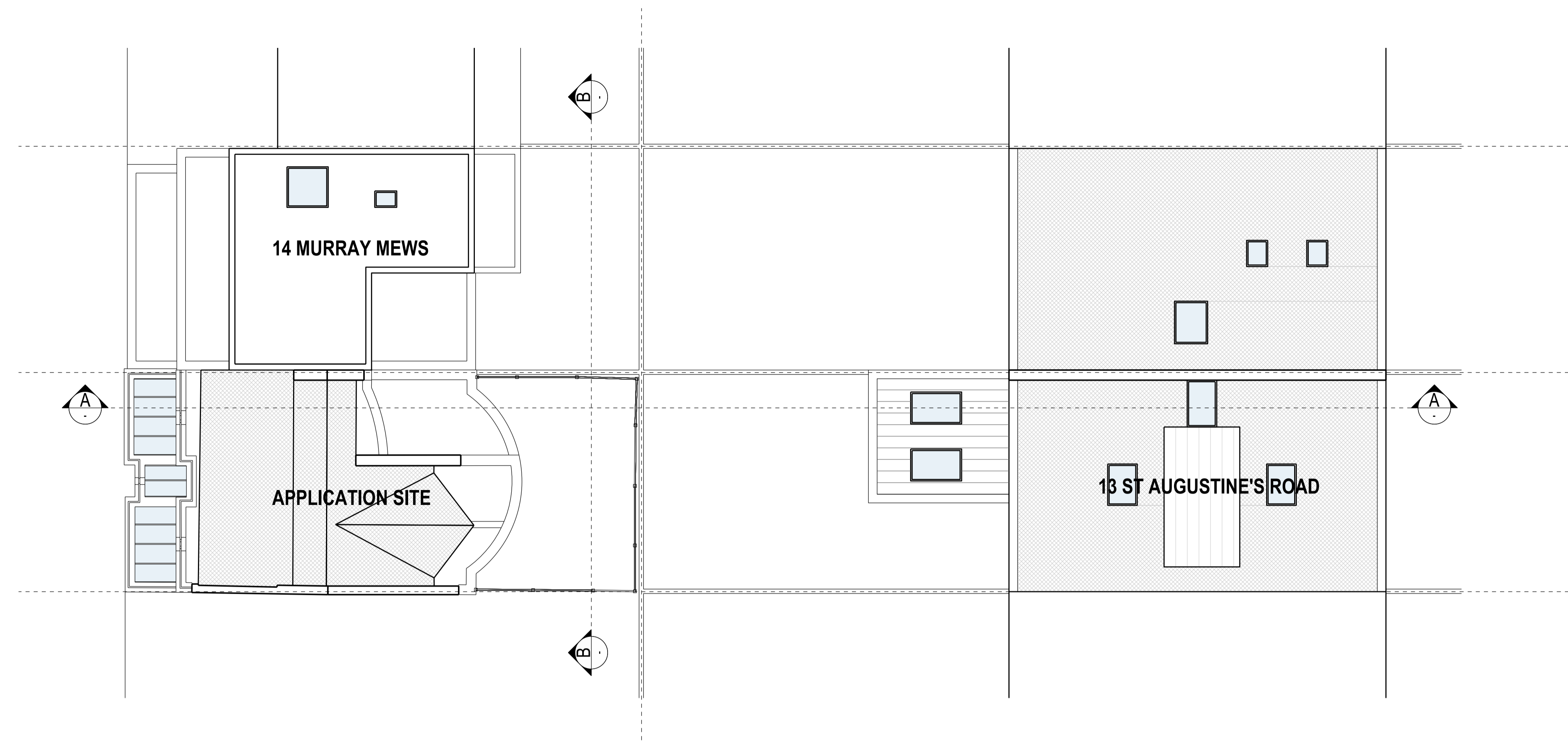
1 EXISTING CONTEXT DRAWINGS - PLAN Scale 1:200 at A3 / 1:100 at A1
