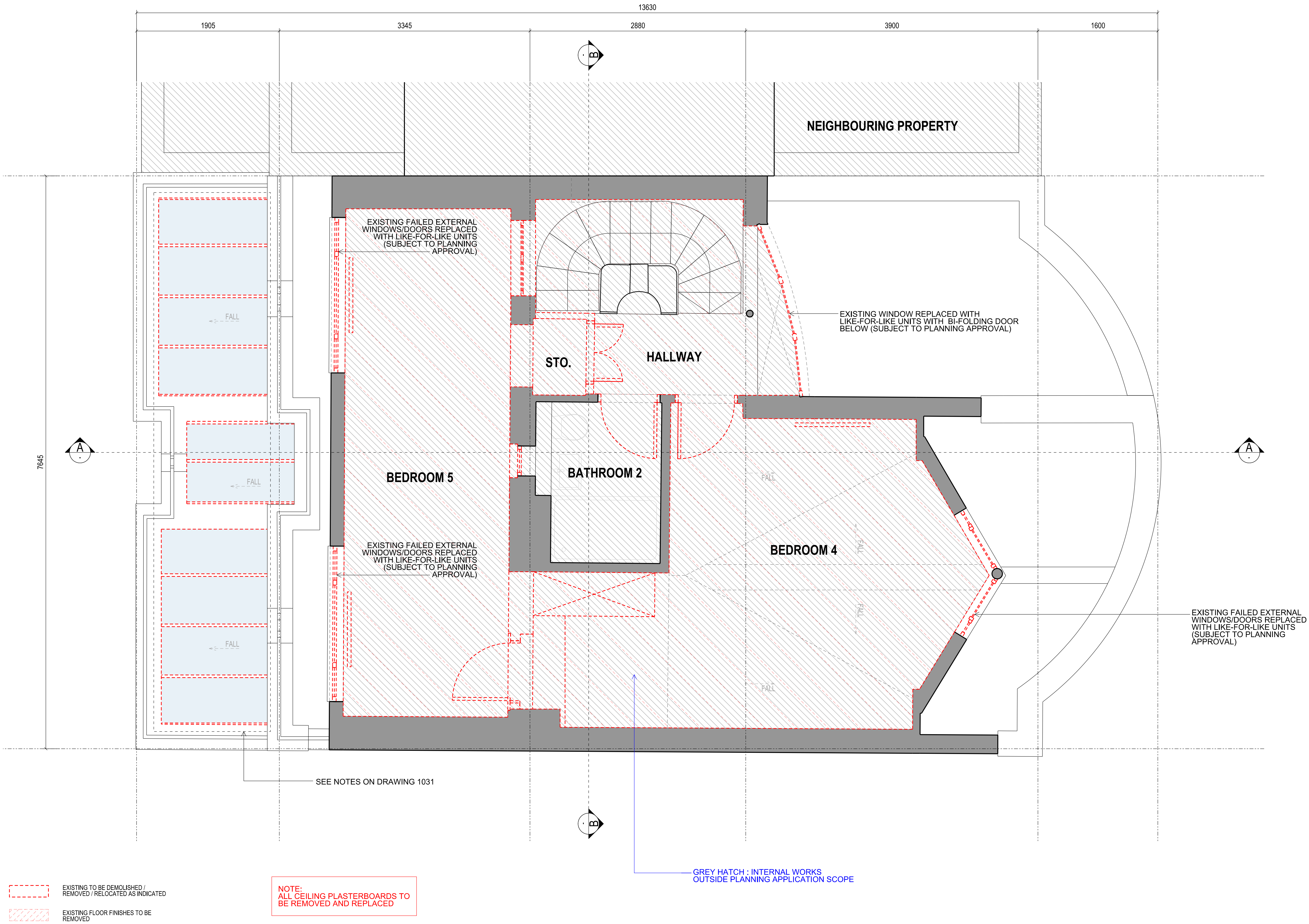
1 EXISTING SECOND FLOOR - DEMOLITION PLAN Scale 1:50 at A3 / 1:25 at A1
