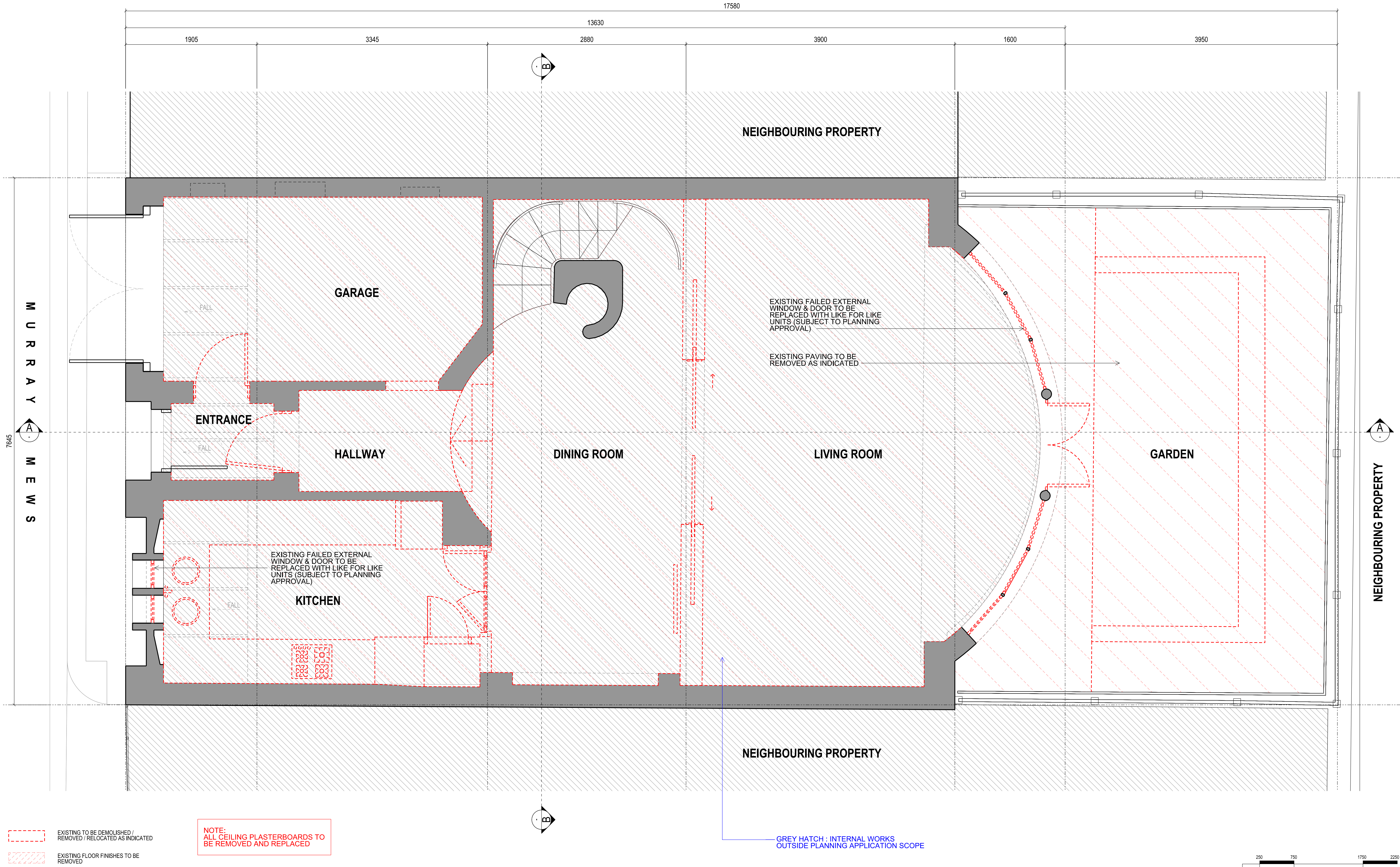
1 EXISTING GROUND FLOOR - DEMOLITION PLAN Scale 1:50 at A3 / 1:25 at A1
