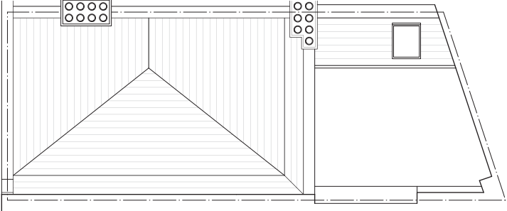
ROOF
