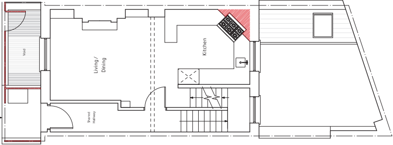
GROUND FLOOR
