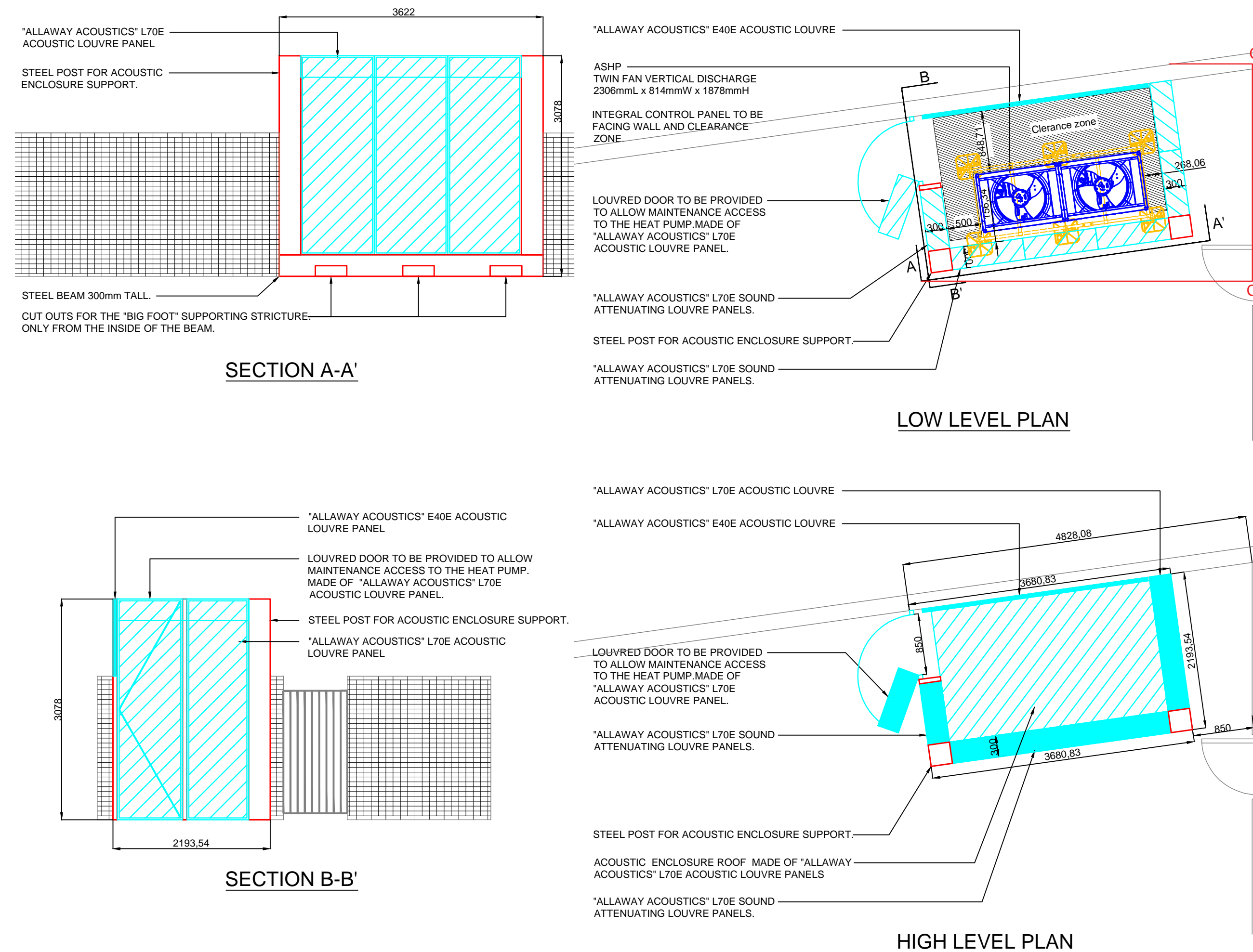
FIGURE 4: AIR SOURCE HEAT PUMP (ASHP) AND ACOUSTIC SCREEN SCALE 1:50
