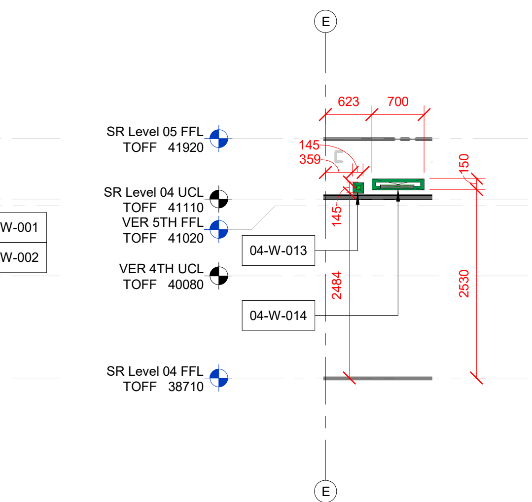
11 Level 04 SR Builderswork Section 11 SCALE: 1 : 50
