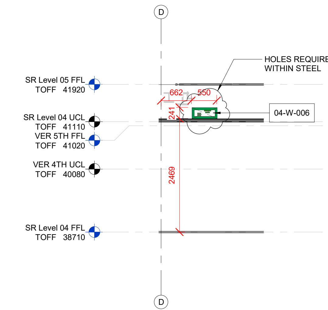
4 Level 04 SR Builderswork Section 4 SCALE: 1 : 50
