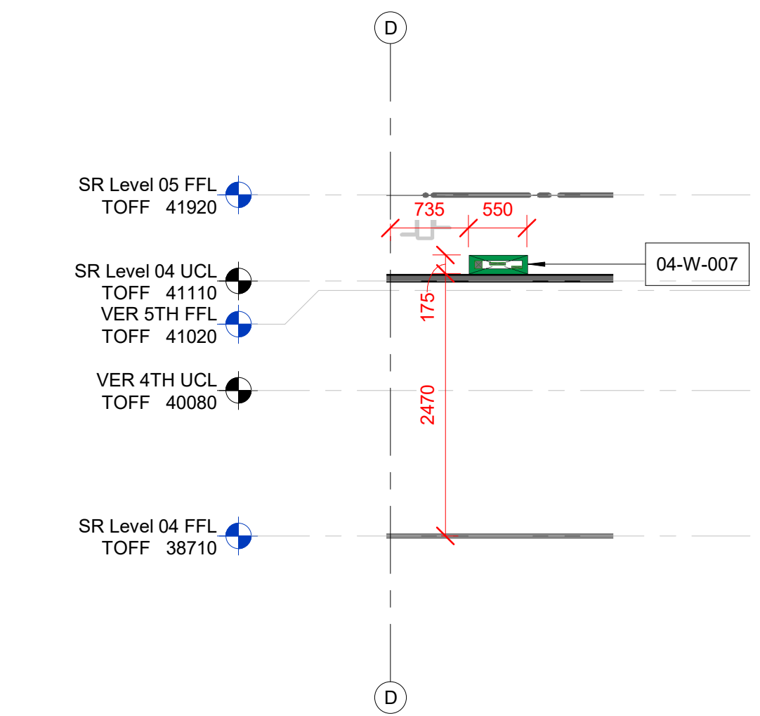
3 Level 04 SR Builderswork Section 3 SCALE: 1 : 50
