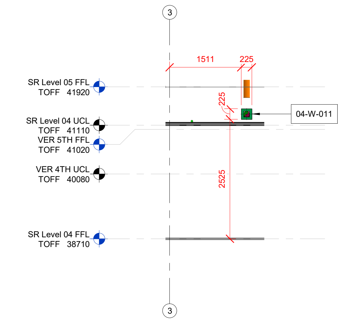
1 Level 04 SR Builderswork Section 1 SCALE: 1 : 50
