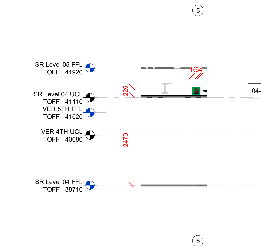
9 Level 04 SR Builderswork Section 9 SCALE: 1 : 50
