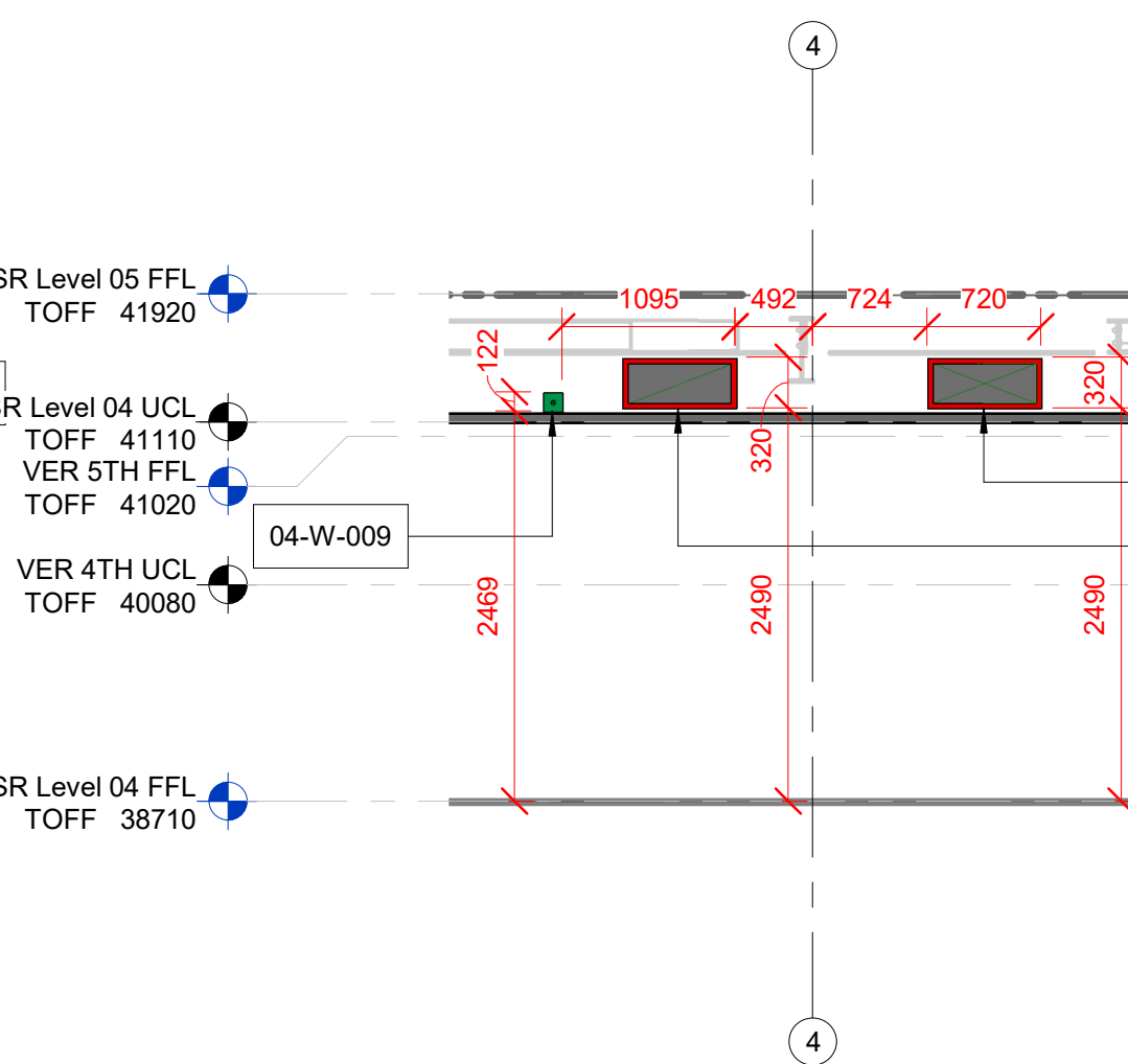
10 Level 04 SR Builderswork Section 10 SCALE: 1 : 50
