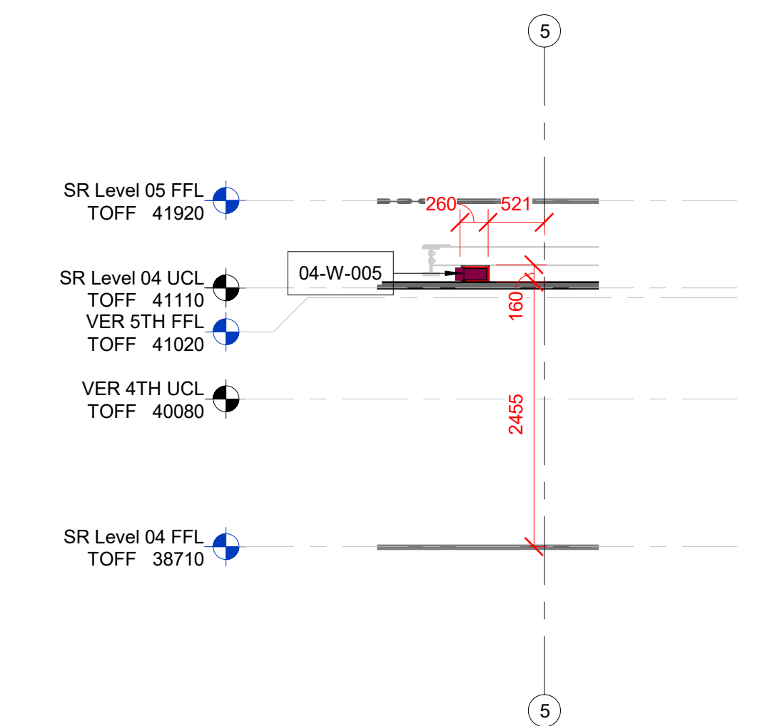
7 Level 04 SR Builderswork Section 7 SCALE: 1 : 50
