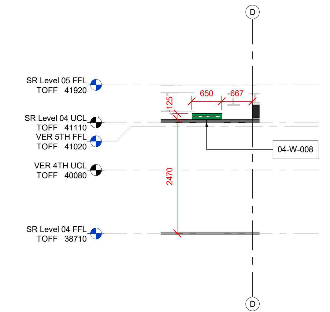
5 Level 04 SR Builderswork Section 5 SCALE: 1 : 50
