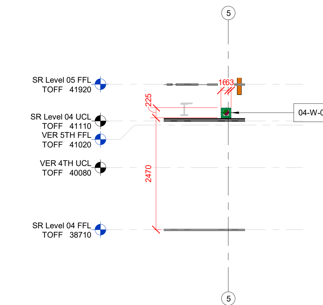
8 Level 04 SR Builderswork Section 8 SCALE: 1 : 50
