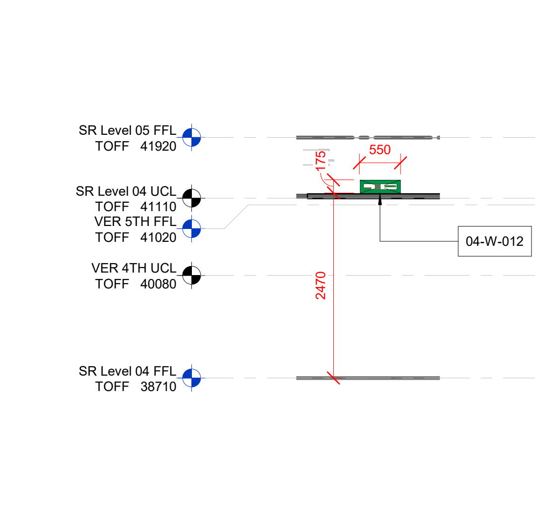
6 Level 04 SR Builderswork Section 6 SCALE: 1 : 50
