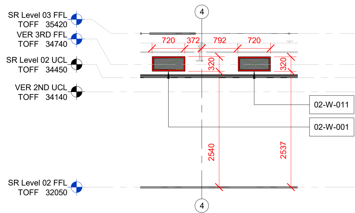
11 Level 02 SR Builderswork Section 11 SCALE: 1 : 50
