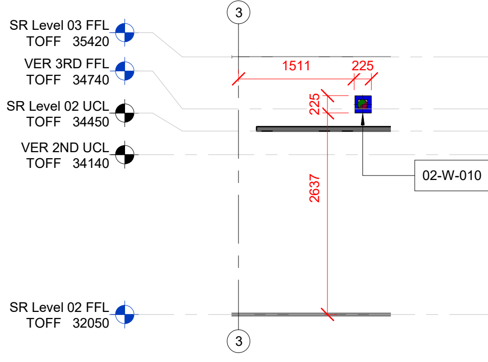
2 Level 02 SR Builderswork Section 2 SCALE: 1 : 50
