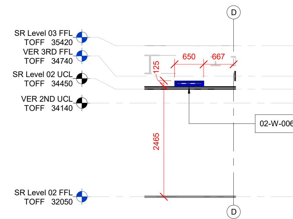
6 Level 02 SR Builderswork Section 6 SCALE: 1 : 50
