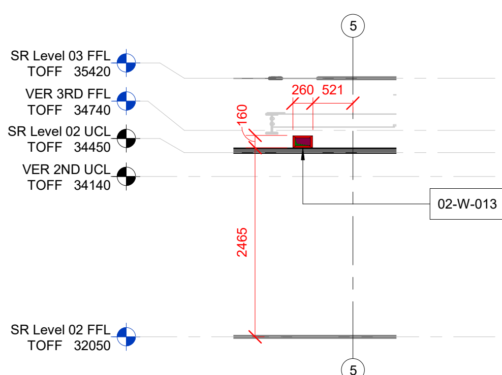
8 Level 02 SR Builderswork Section 8 SCALE: 1 : 50
