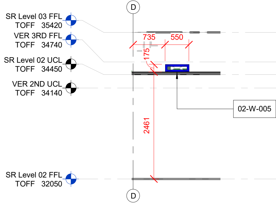
4 Level 02 SR Builderswork Section 4 SCALE: 1 : 50
