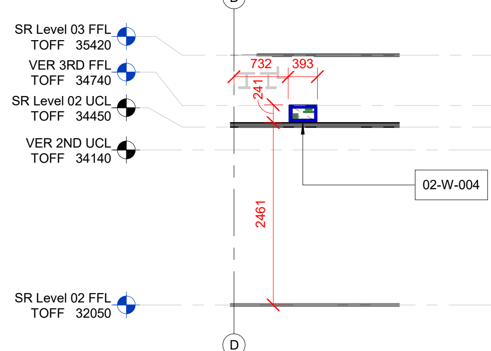
5 Level 02 SR Builderswork Section 5 SCALE: 1 : 50
