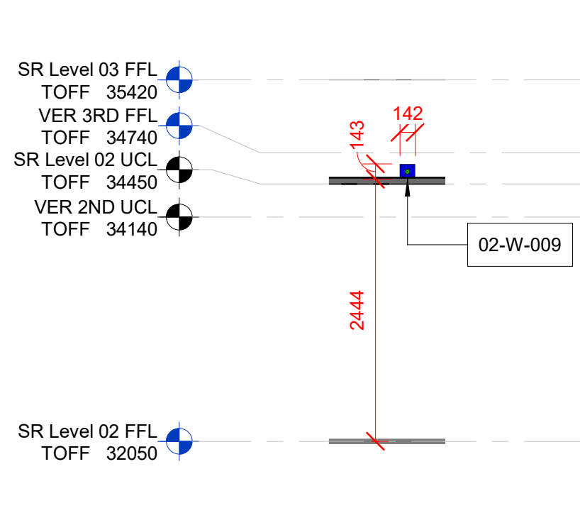
3 Level 02 SR Builderswork Section 3 SCALE: 1 : 50
