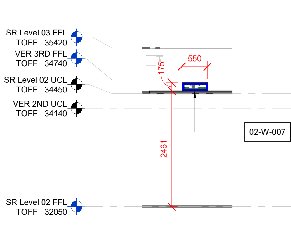
7 Level 02 SR Builderswork Section 7 SCALE: 1 : 50
