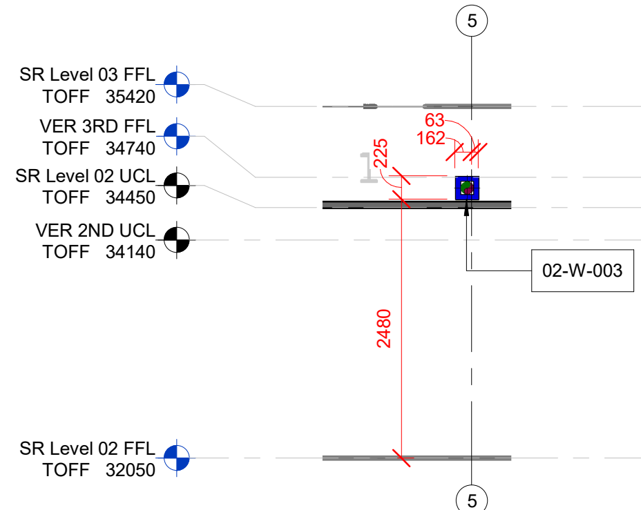
9 Level 02 SR Builderswork Section 9 SCALE: 1 : 50
