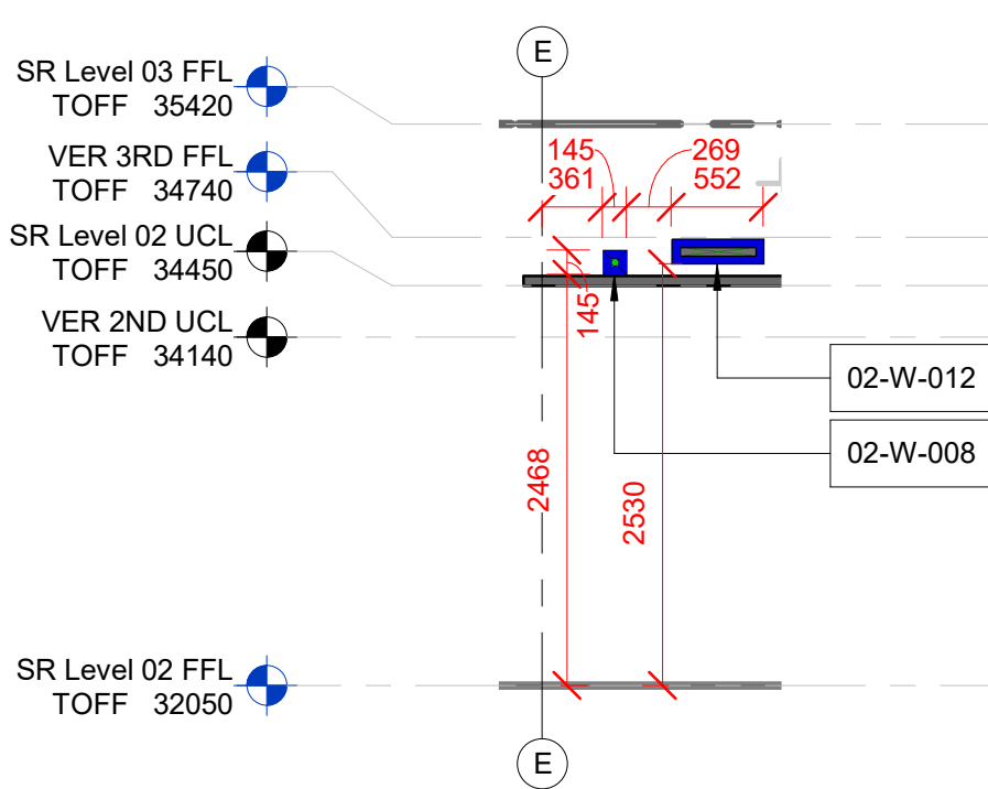
1 Level 02 SR Builderswork Section 1 SCALE: 1 : 50
