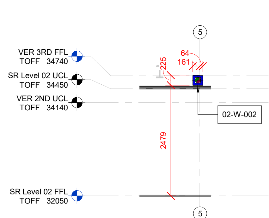
10 Level 02 SR Builderswork Section 10 SCALE: 1 : 50
