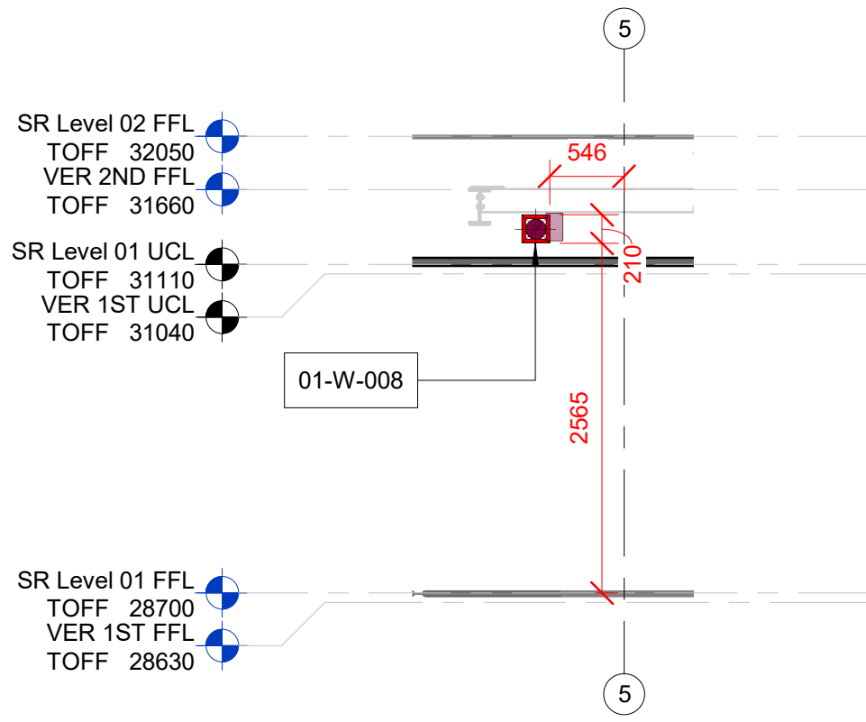
1 Level 01 SR Builderswork Section 1 SCALE: 1 : 50
