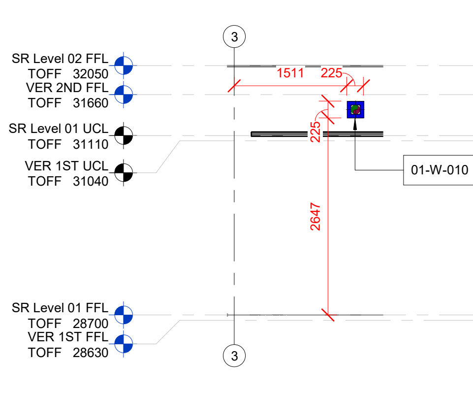
11 Level 01 SR Builderswork Section 11 SCALE: 1 : 50
