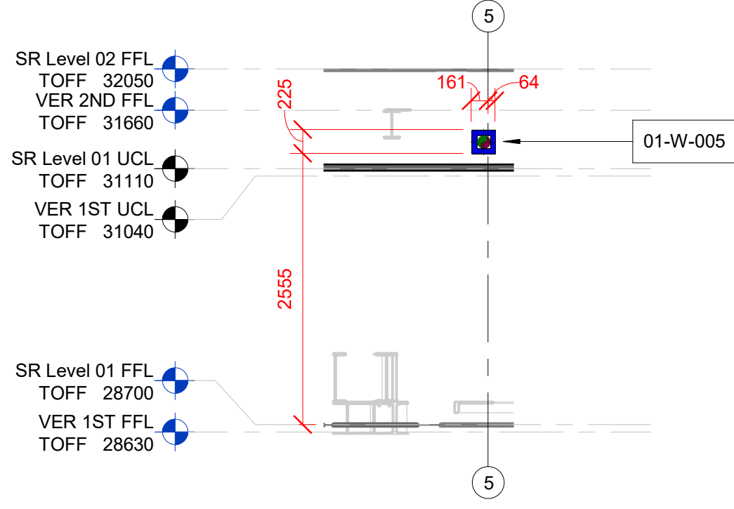
6 Level 01 SR Builderswork Section 6 SCALE: 1 : 50
