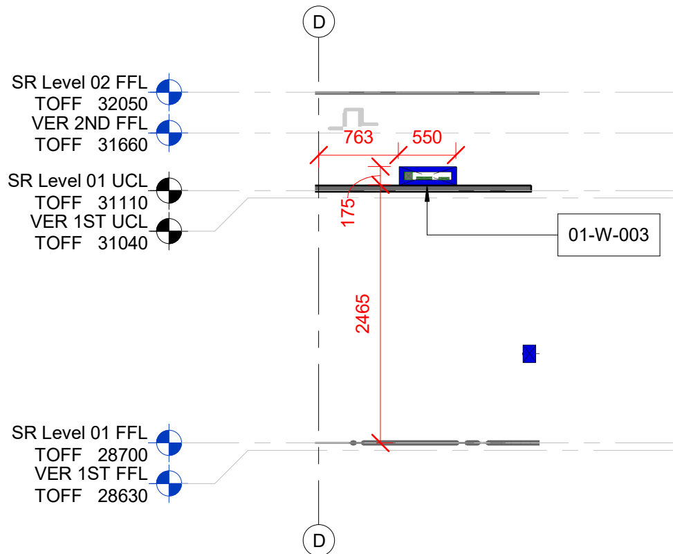
9 Level 01 SR Builderswork Section 9 SCALE: 1 : 50
