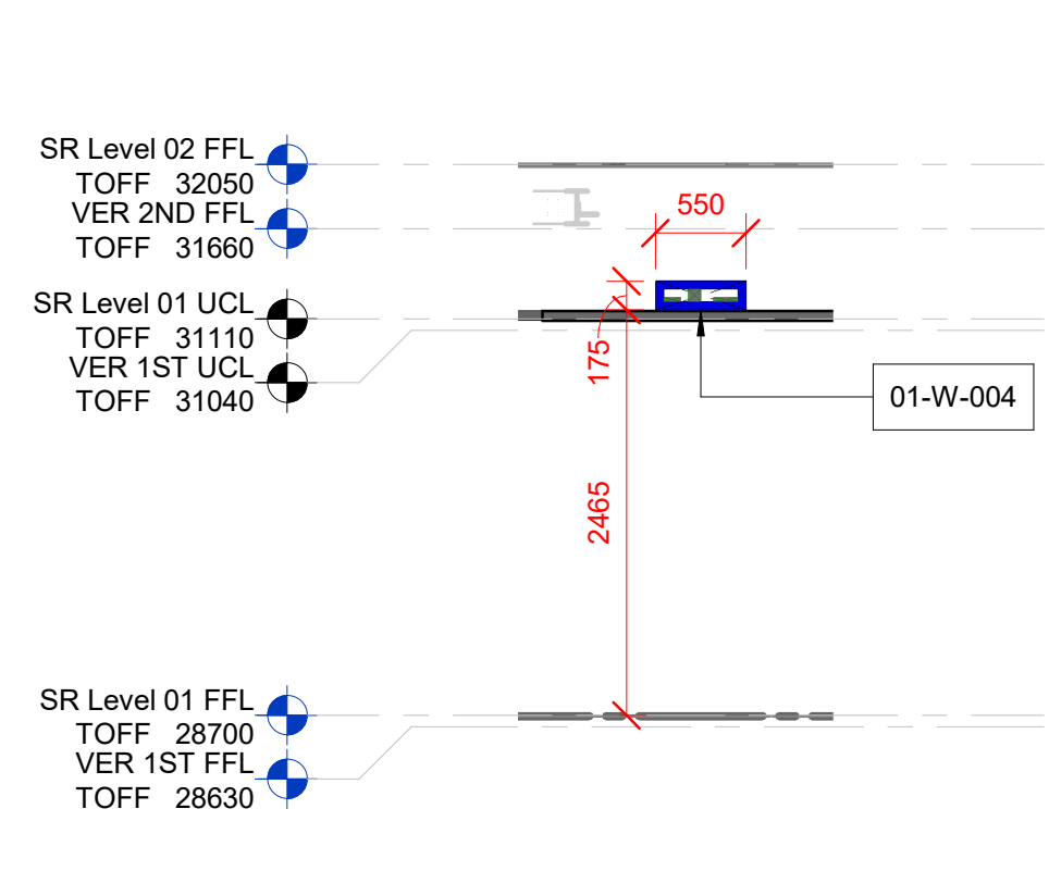
4 Level 01 SR Builderswork Section 4 SCALE: 1 : 50
