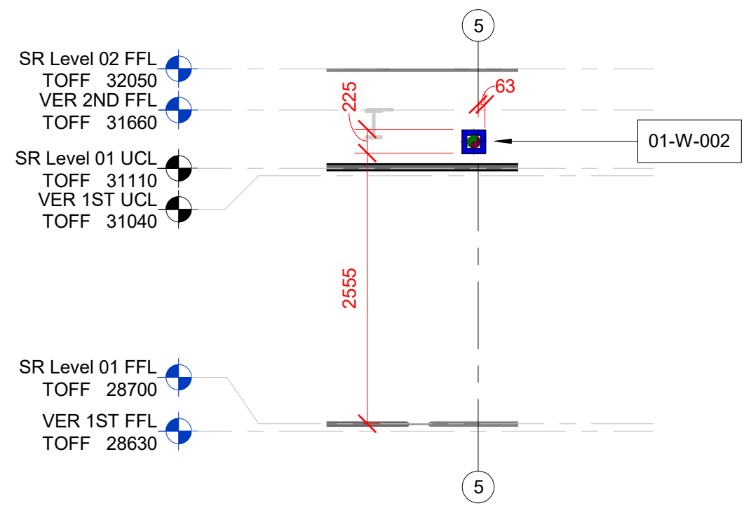
5 Level 01 SR Builderswork Section 5 SCALE: 1 : 50
