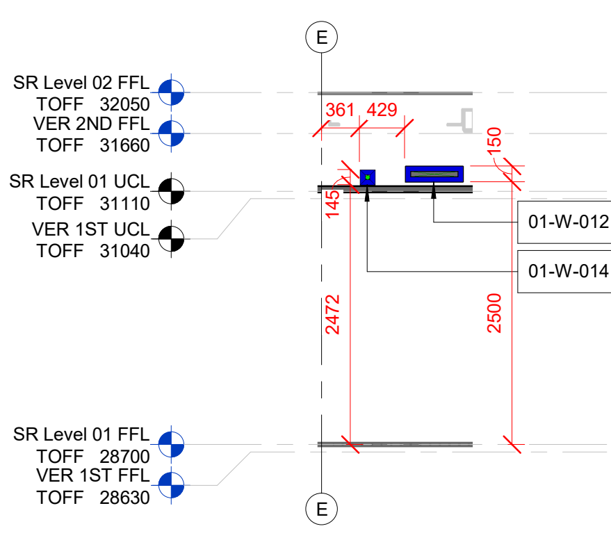
10 Level 01 SR Builderswork Section 10 SCALE: 1 : 50
