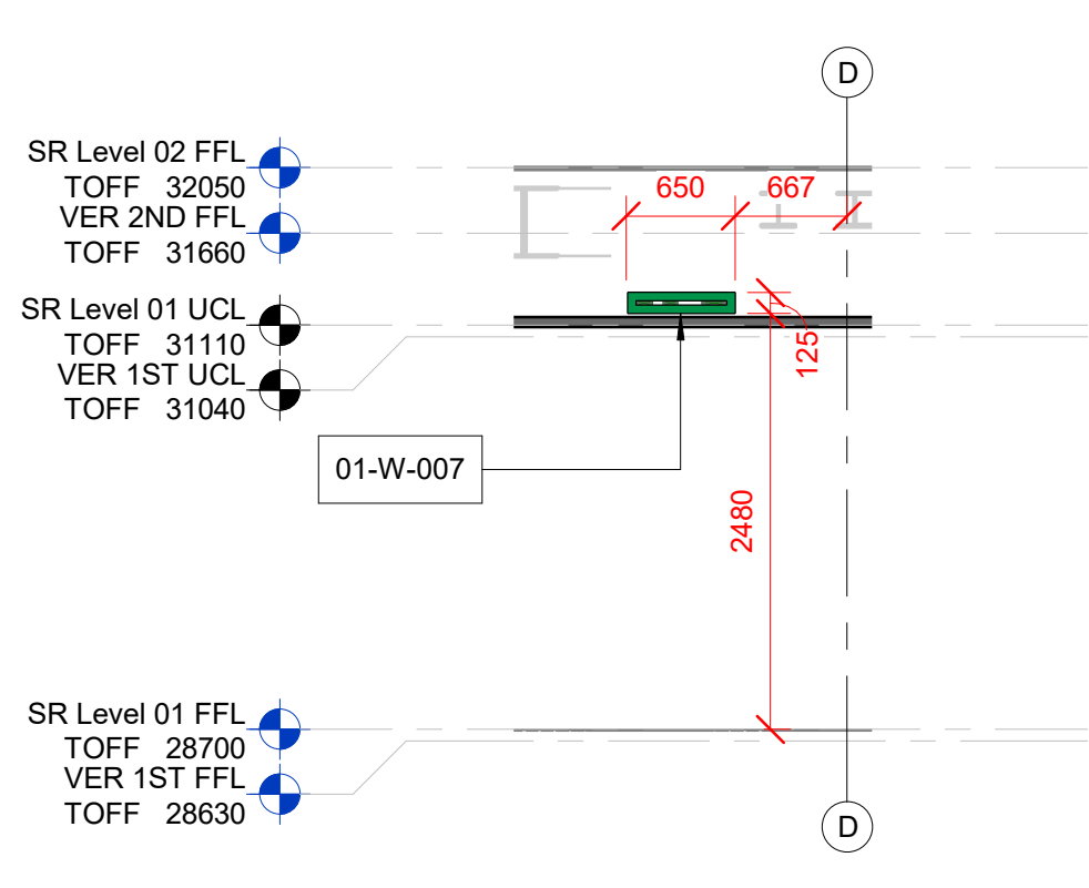
2 Level 01 SR Builderswork Section 2 SCALE: 1 : 50
