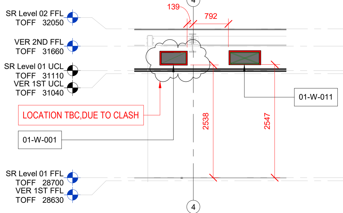
7 Level 01 SR Builderswork Section 7 SCALE: 1 : 50
