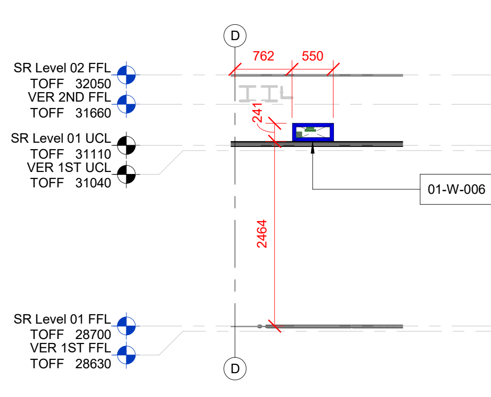
3 Level 01 SR Builderswork Section 3 SCALE: 1 : 50
