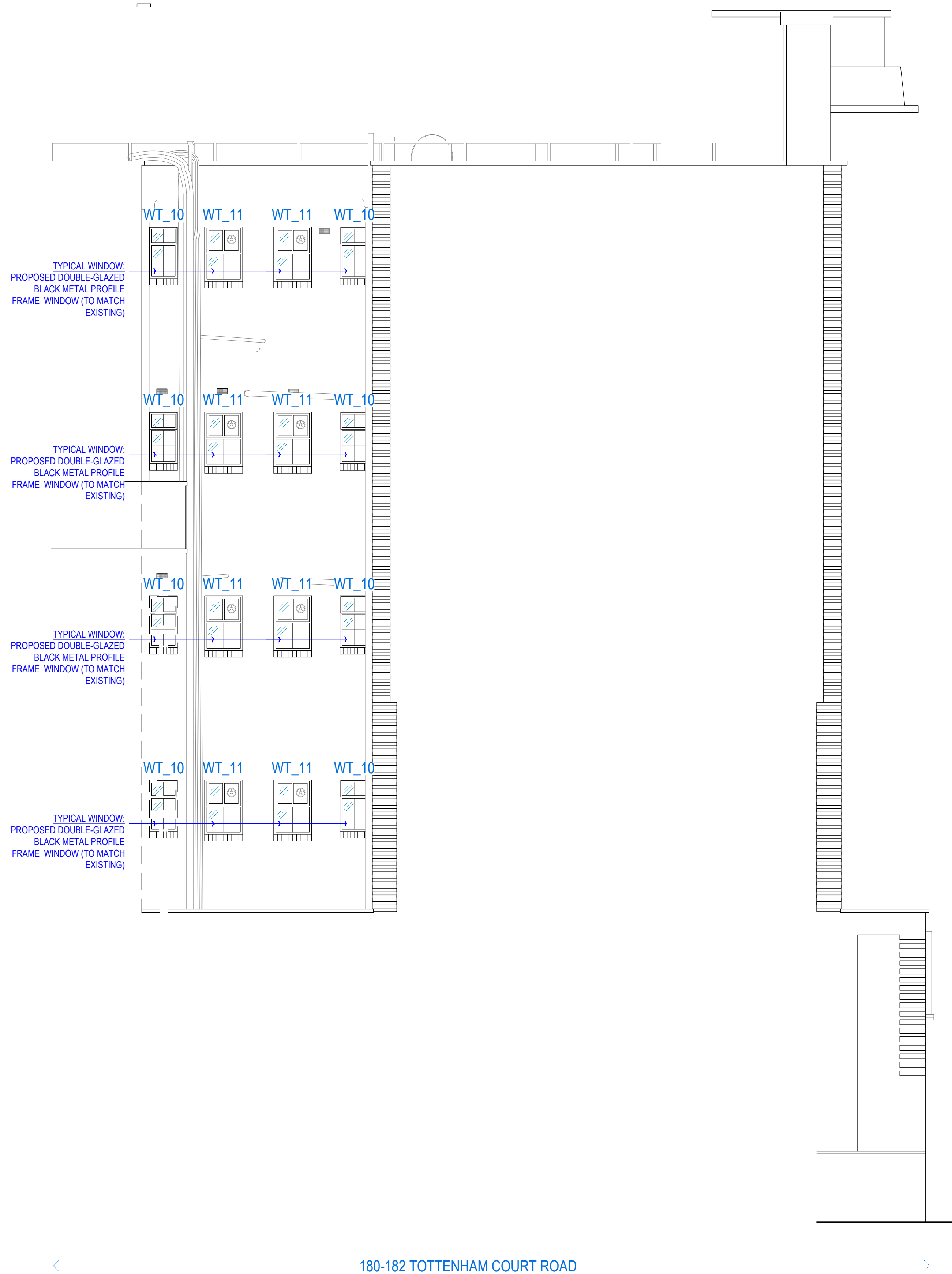
ELEVATION 5 - PROPOSED SIDE ELEVATION (SOUTH-EAST)
