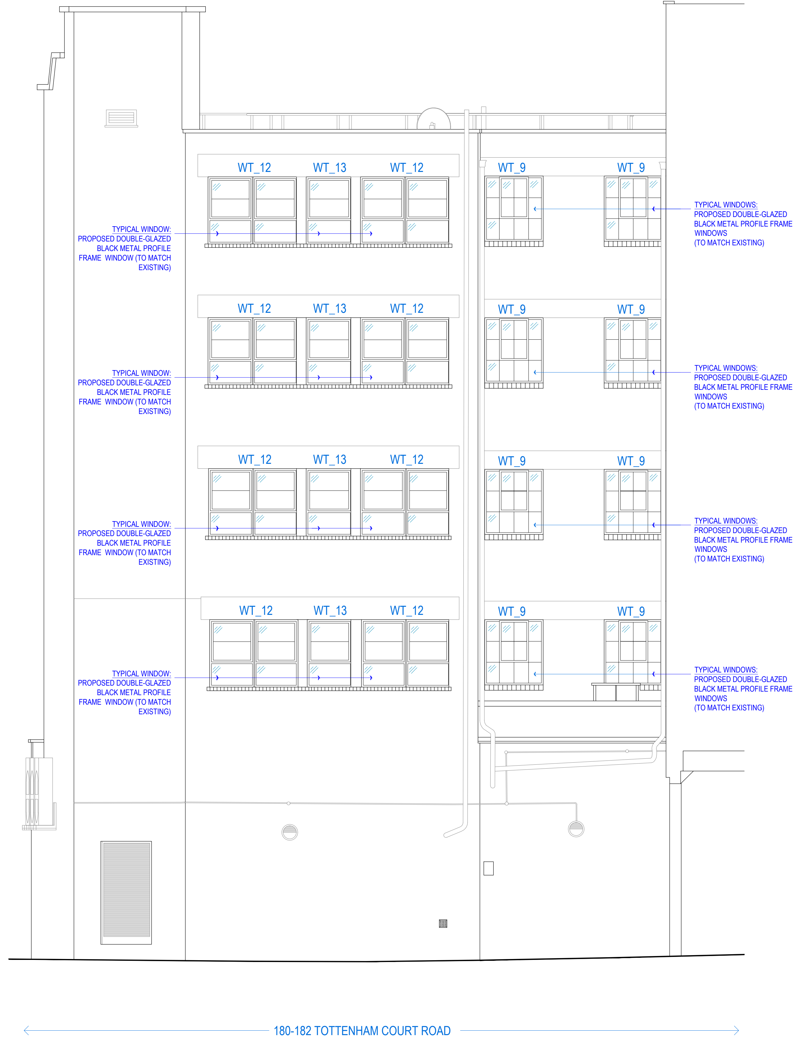
ELEVATION 6 - PROPOSED SIDE ELEVATION (NORTH-WEST)
