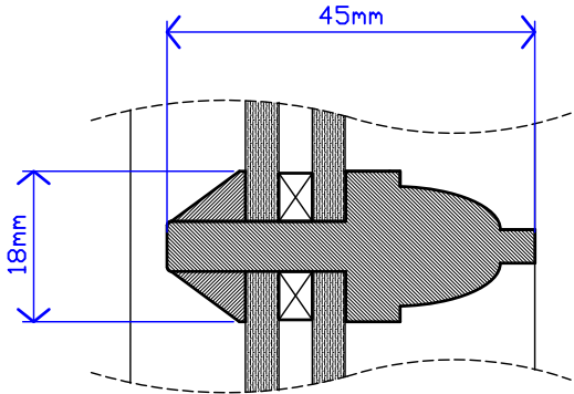
DETAIL OF GLAZING BAR SHOWN AT 1:1 SCALE
