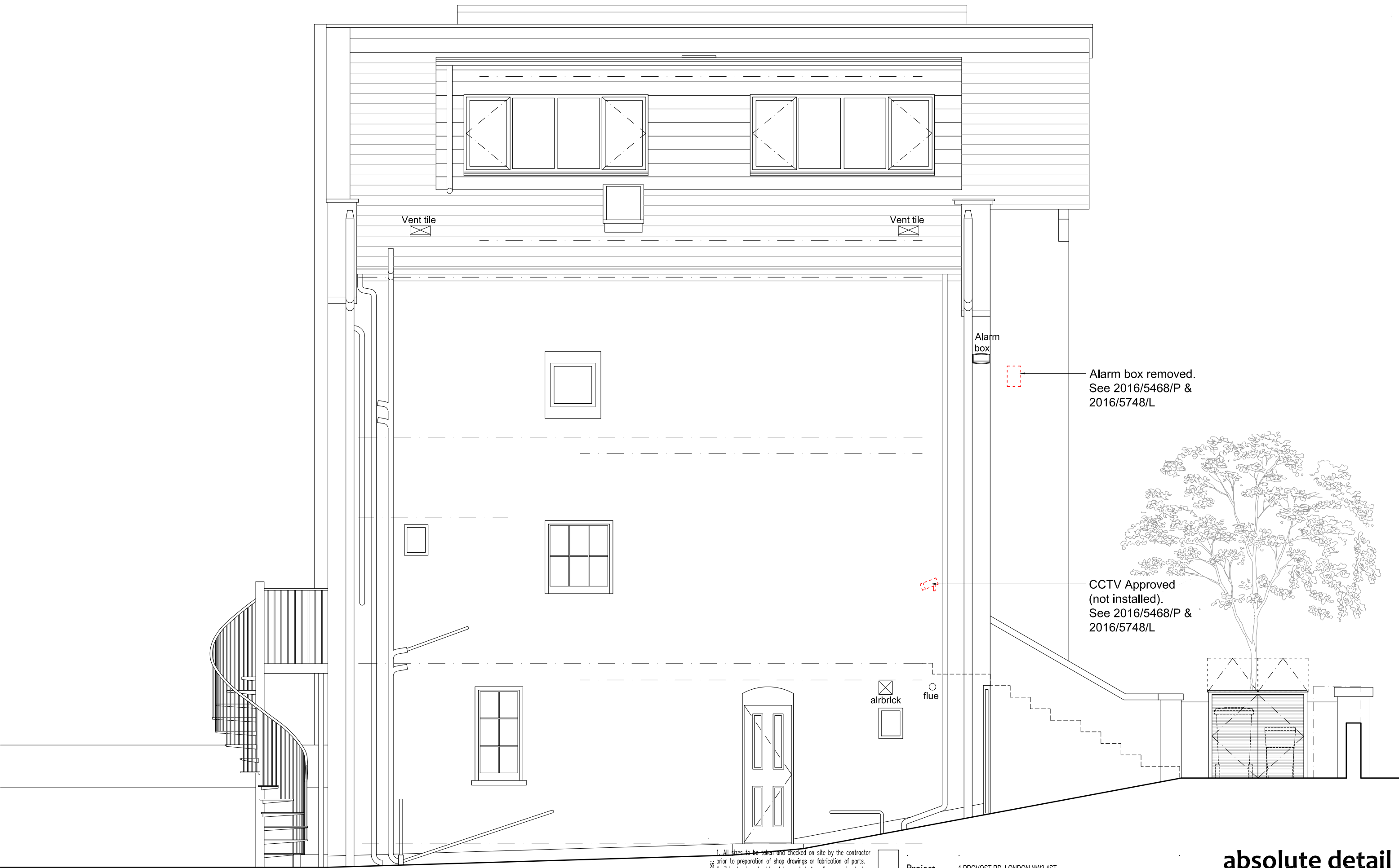
Flank (side) Elevation as Existing
