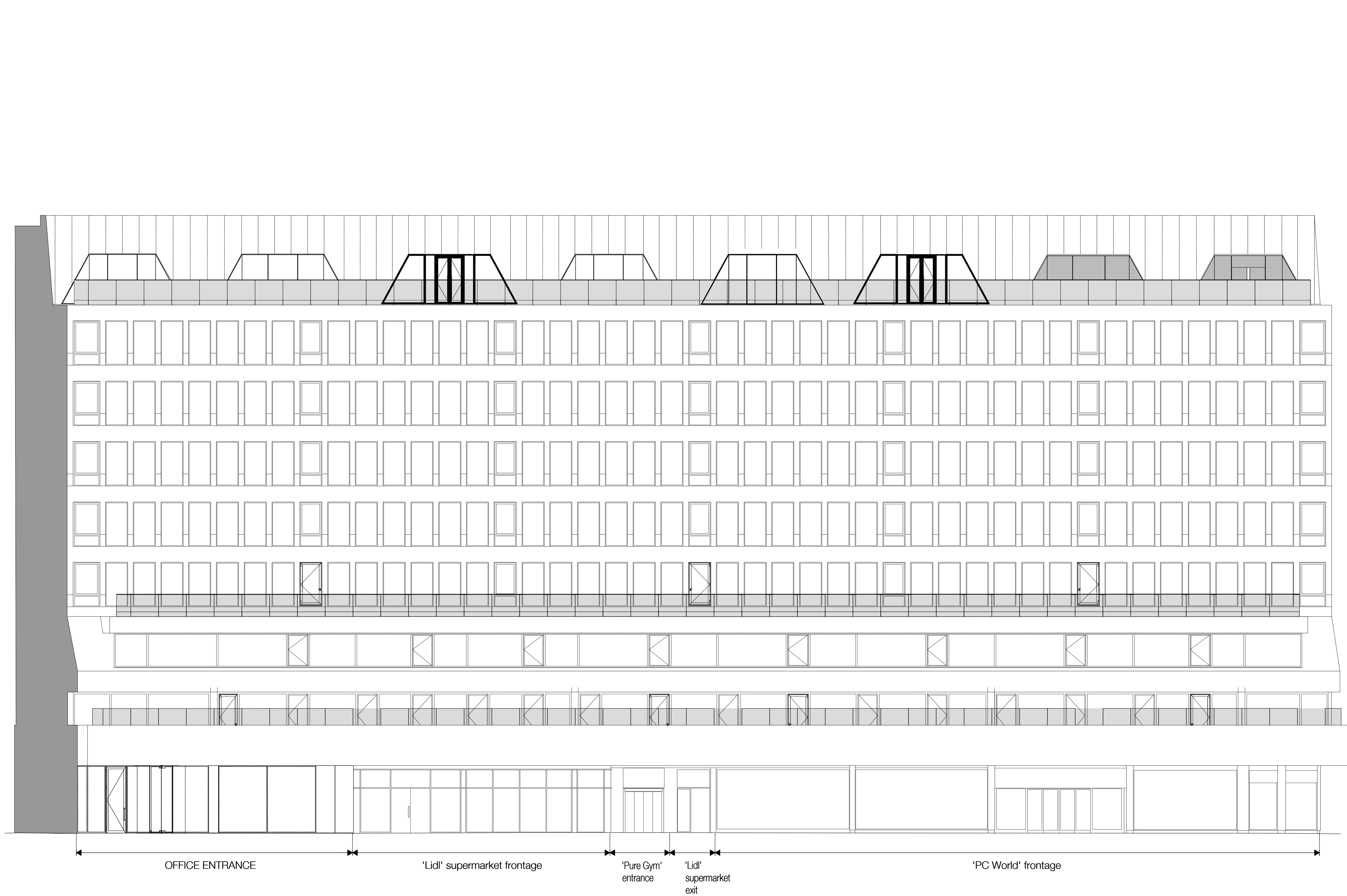
01 EXISTING WEST ELEVATION - TOTTENHAM COURT ROAD PL020 SCALE: 1:100 @ A1
