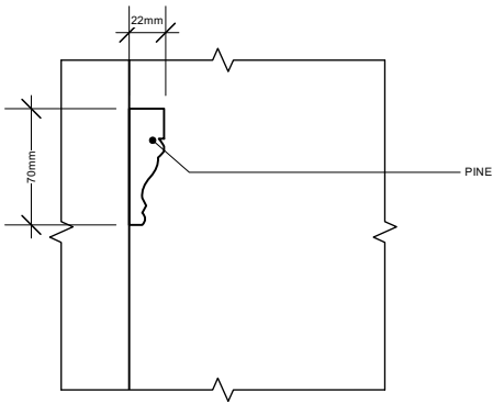
PROPOSED DETAIL - ARCHITRAVE 2 (1:5) (The Duchy Victorian) (Second & Third Floor)
