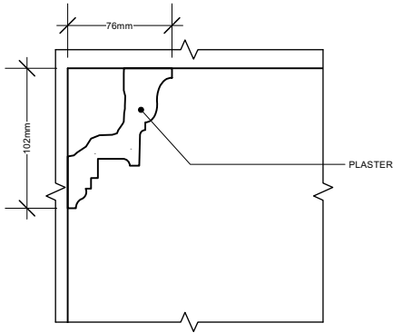
PROPOSED DETAIL - CORNICE 4 (1:5) (Small Dentil Plaster) (Second & Third Floor)
