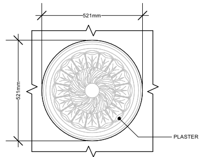
PROPOSED DETAIL - CEILING ROSE 4 (1:50) (Date Leaf Victorian) (Second & Third Floor)
