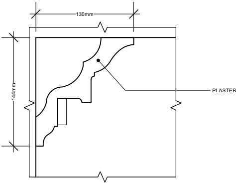
PROPOSED DETAIL - CORNICE 3 (1:5) (Victorian Large Dentil Plaster) (First Floor)
