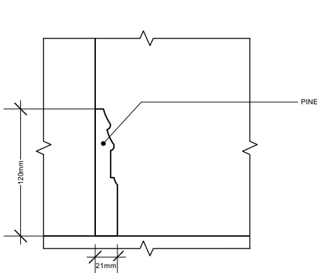
PROPOSED DETAIL - SKIRTING 2 (1:5) (The Ampleforth Victorian) (Lower Ground, Second & Third Floor)
