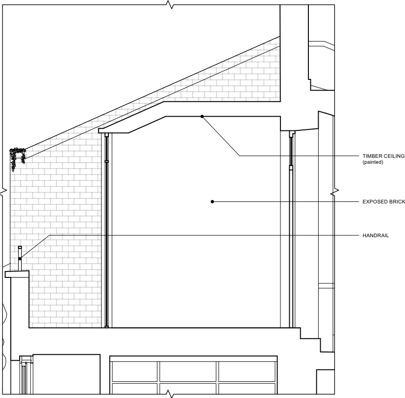
SUNROOM - SECTION (1:50)
