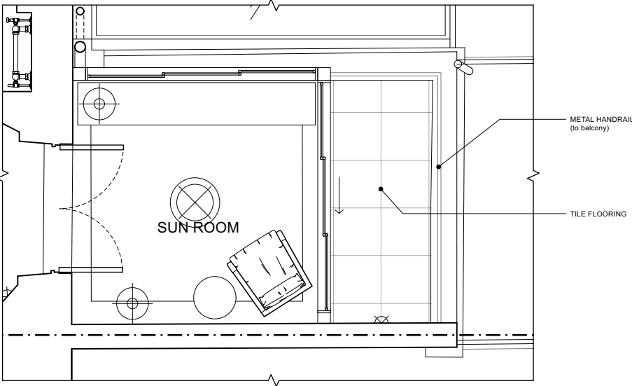
SUNROOM - PLAN (1:50)
