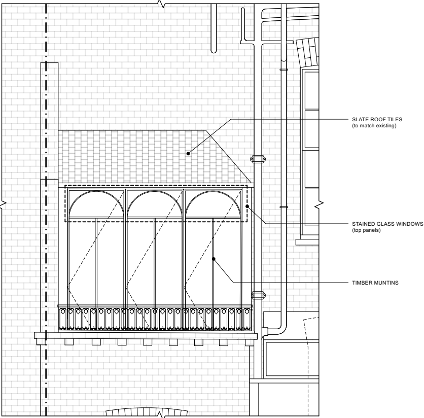
SUNROOM - REAR ELEVATION (1:50)
