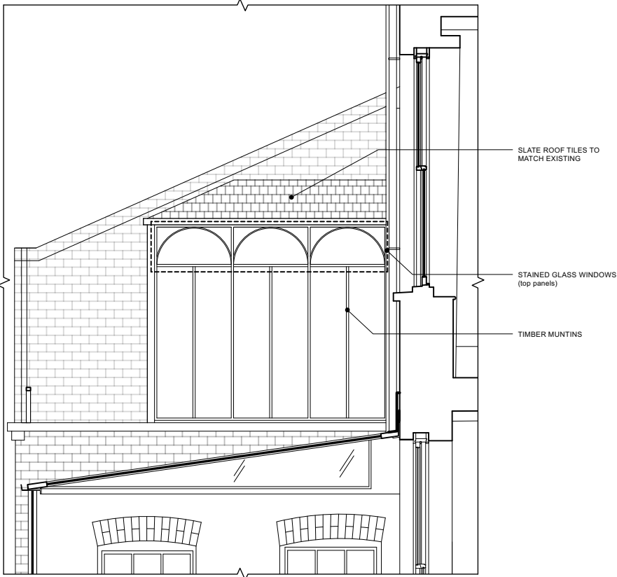
SUNROOM - SIDE ELEVATION (1:50)
