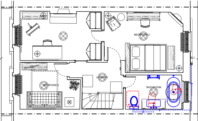
PROPOSED DRAINAGE - THIRD FLOOR (1:100)
