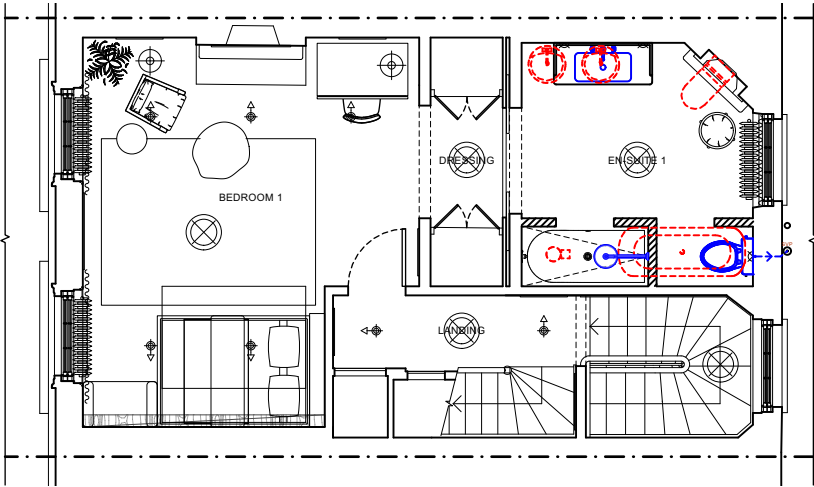
PROPOSED DRAINAGE - SECOND FLOOR (1:100)
