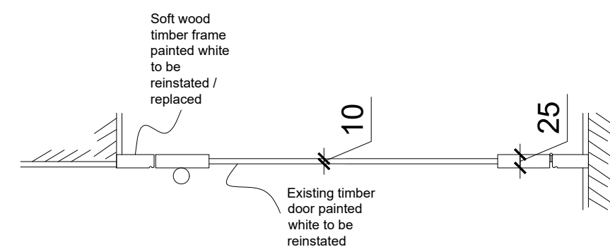
HORIZONTAL SECTION (CUPBOARD DOOR)
