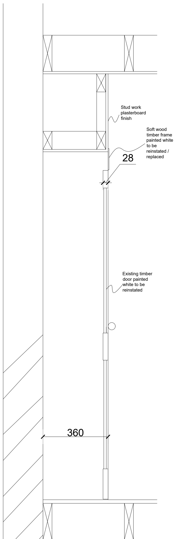
VERTICAL SECTION
